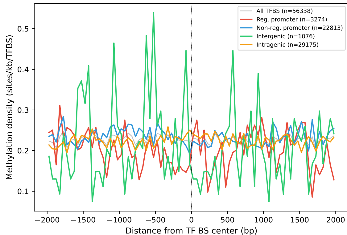
All 4mC T1
