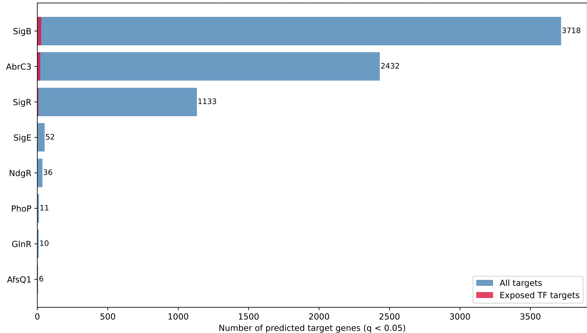
FIMO-predicted targets per TF (promoter \pm 500 bp)
