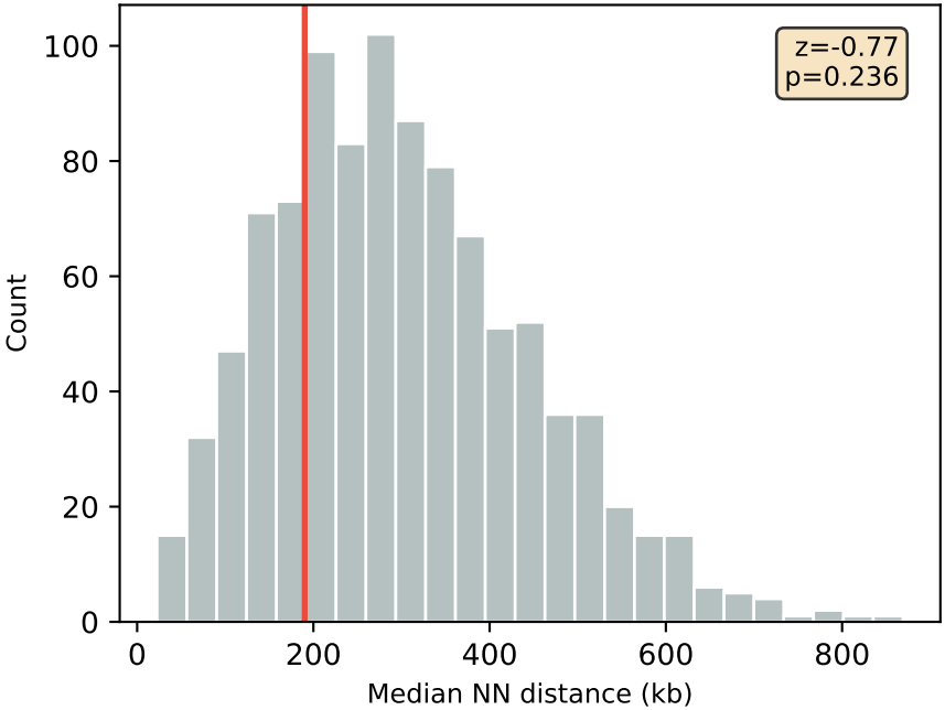
B. Permutation Test (Genomic Clustering)
