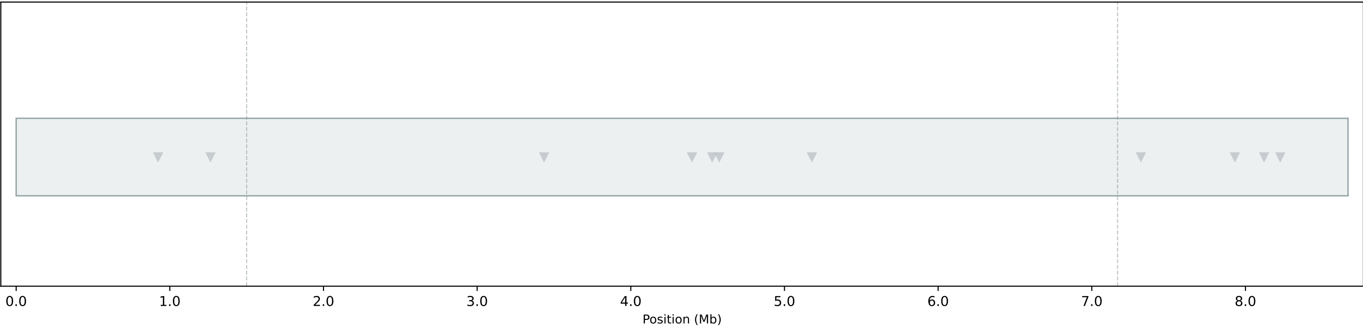
A. Genomic Distribution of 62 Exposed Regulators
