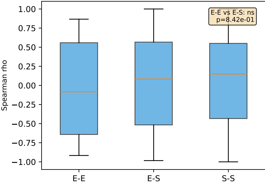
C. Co-expression Comparison
