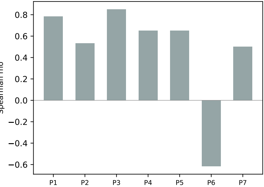
E. TCS Pair Correlations
