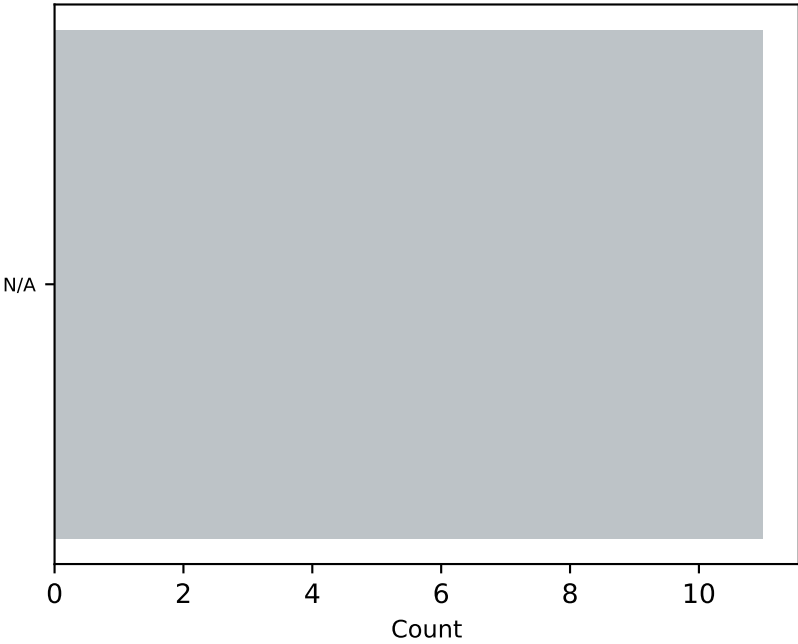
D. Coordination Type (T3)
