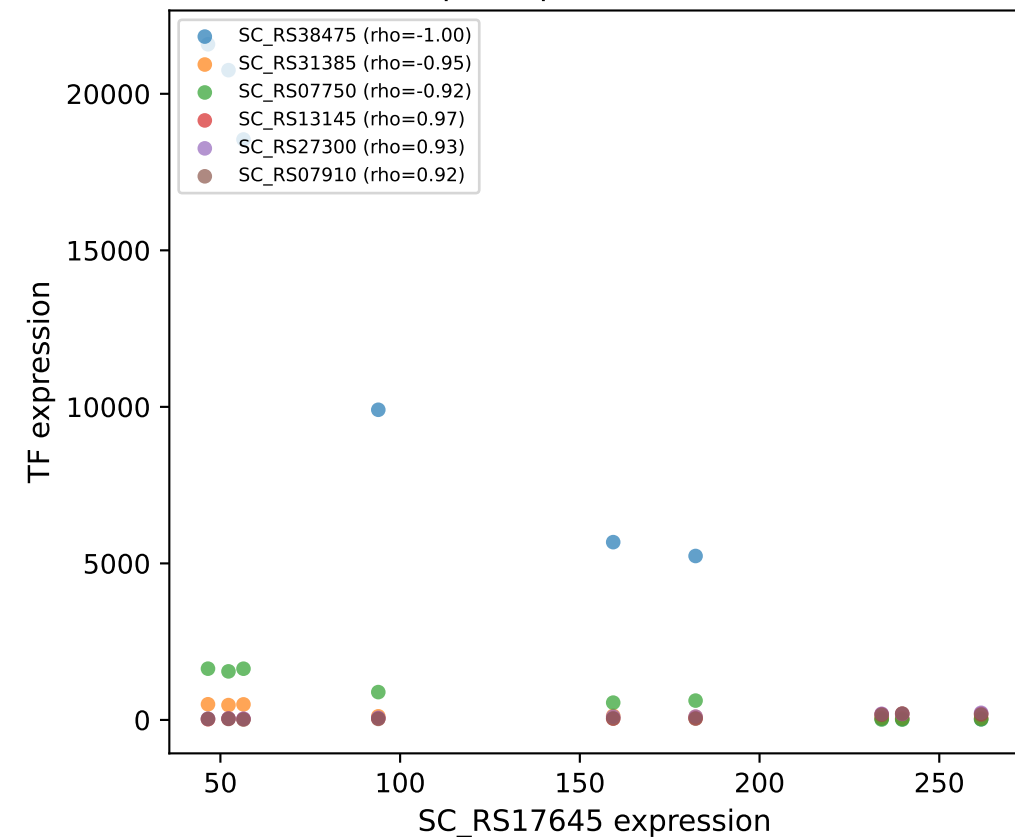
C) Example exposed TF correlations
