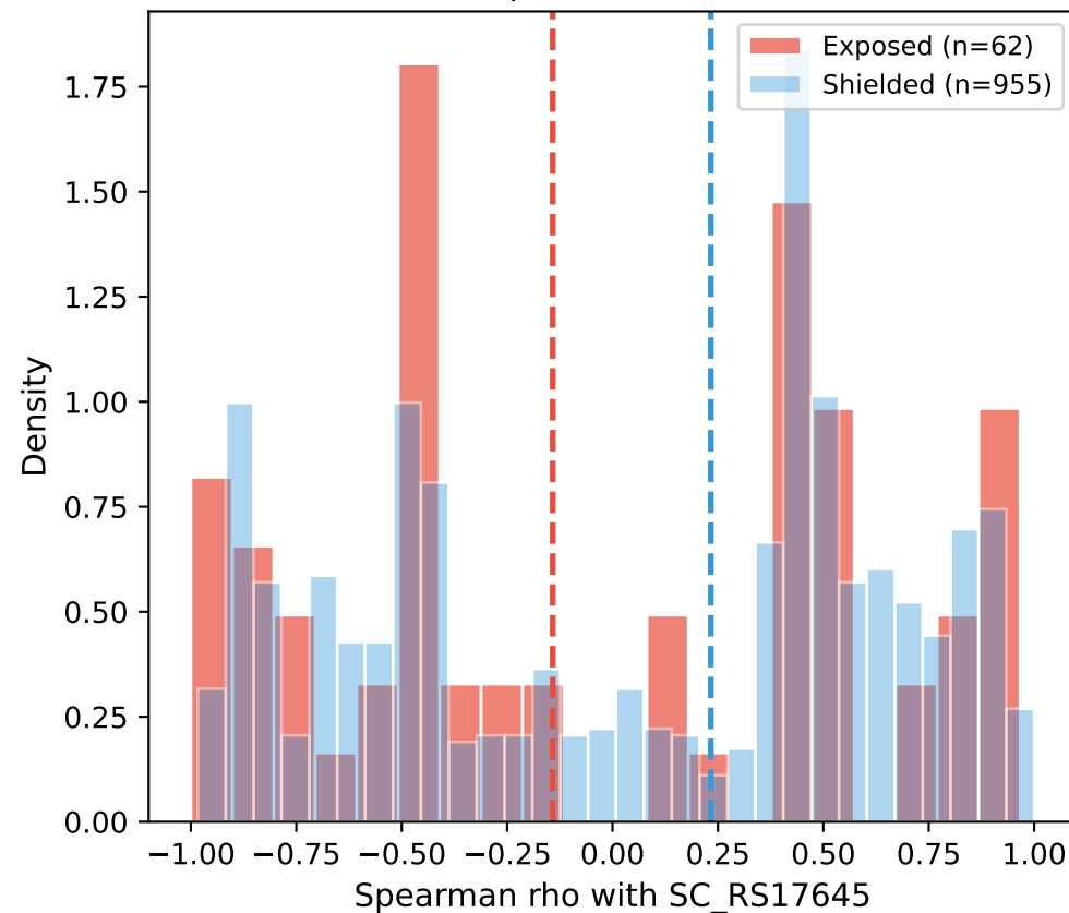
A) MTase-TF expression correlation
