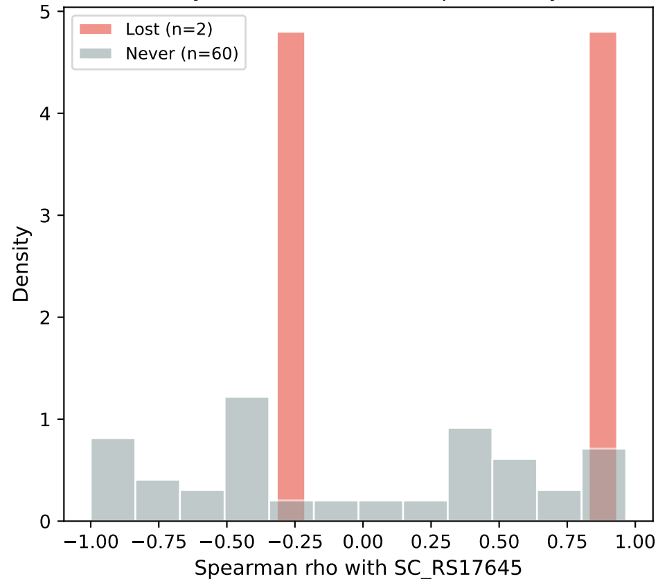
B) By AAGCCCG status (exposed only)
