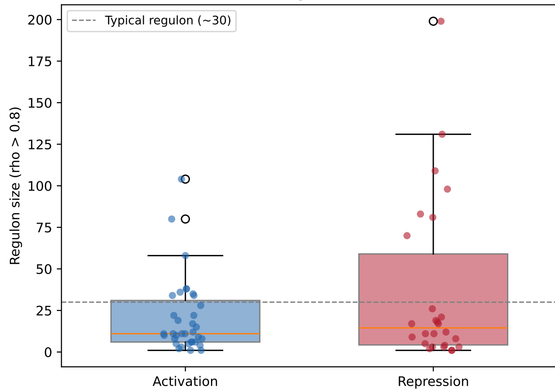
Per-TF regulon size MWU p=0.743
