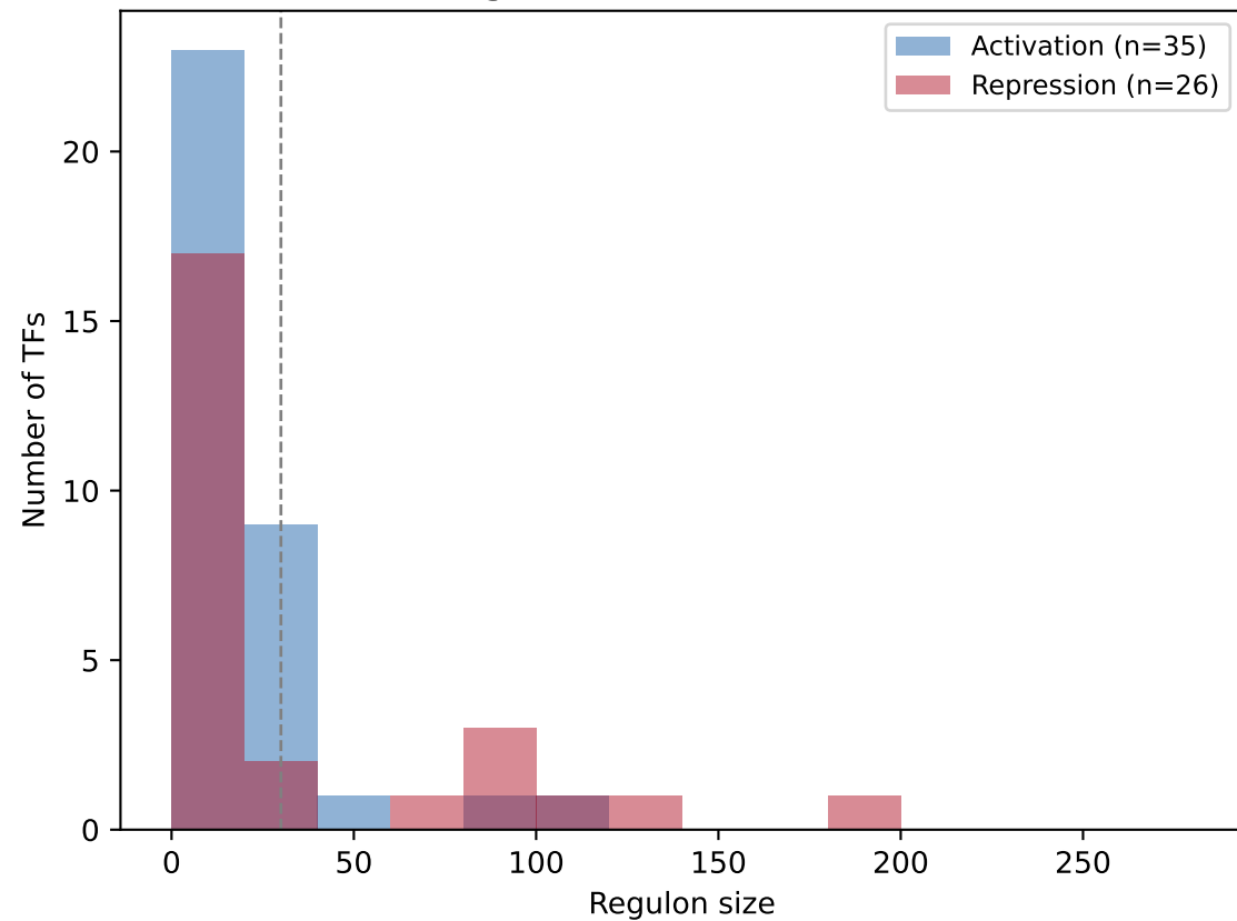
Regulon size distribution
