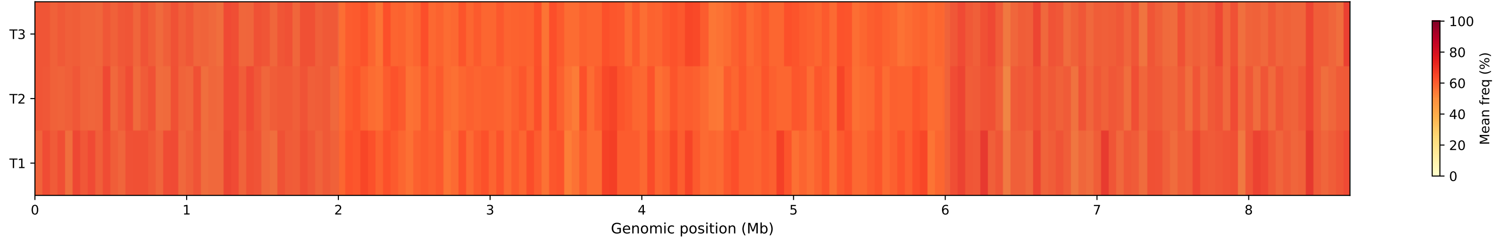
6mA mean methylation frequency (%) - 50kb windows
