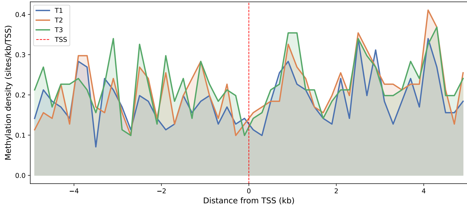
6mA methylation profile around TSS (Regulatory genes)
