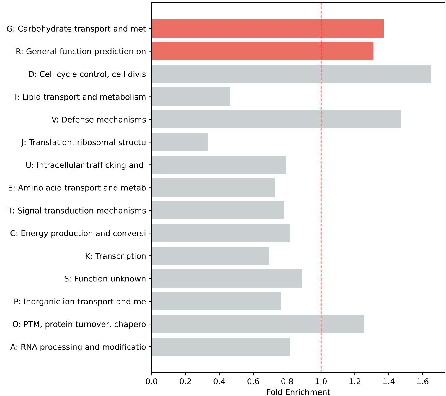
Negative Correlation Genes (n=89) Methyl↔Expr opposite direction
