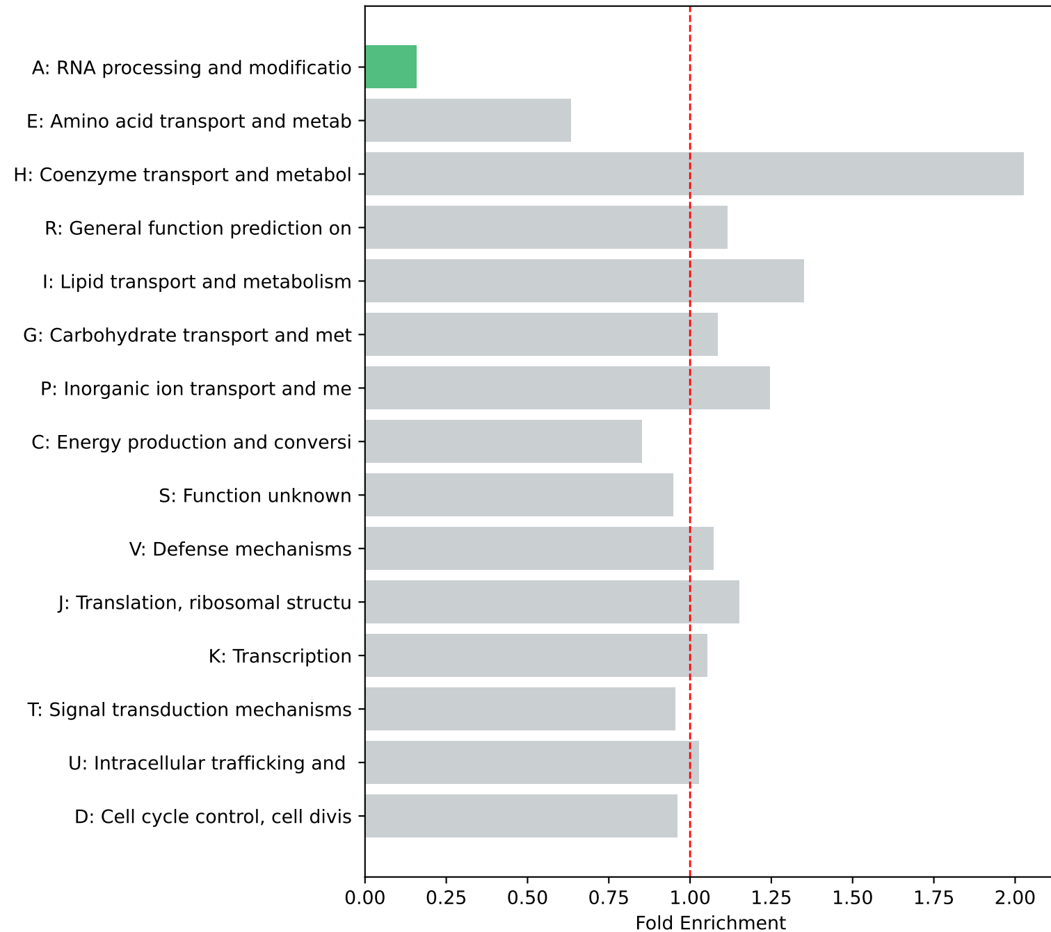
Positive Correlation Genes (n=153) Methyl↔Expr same direction
