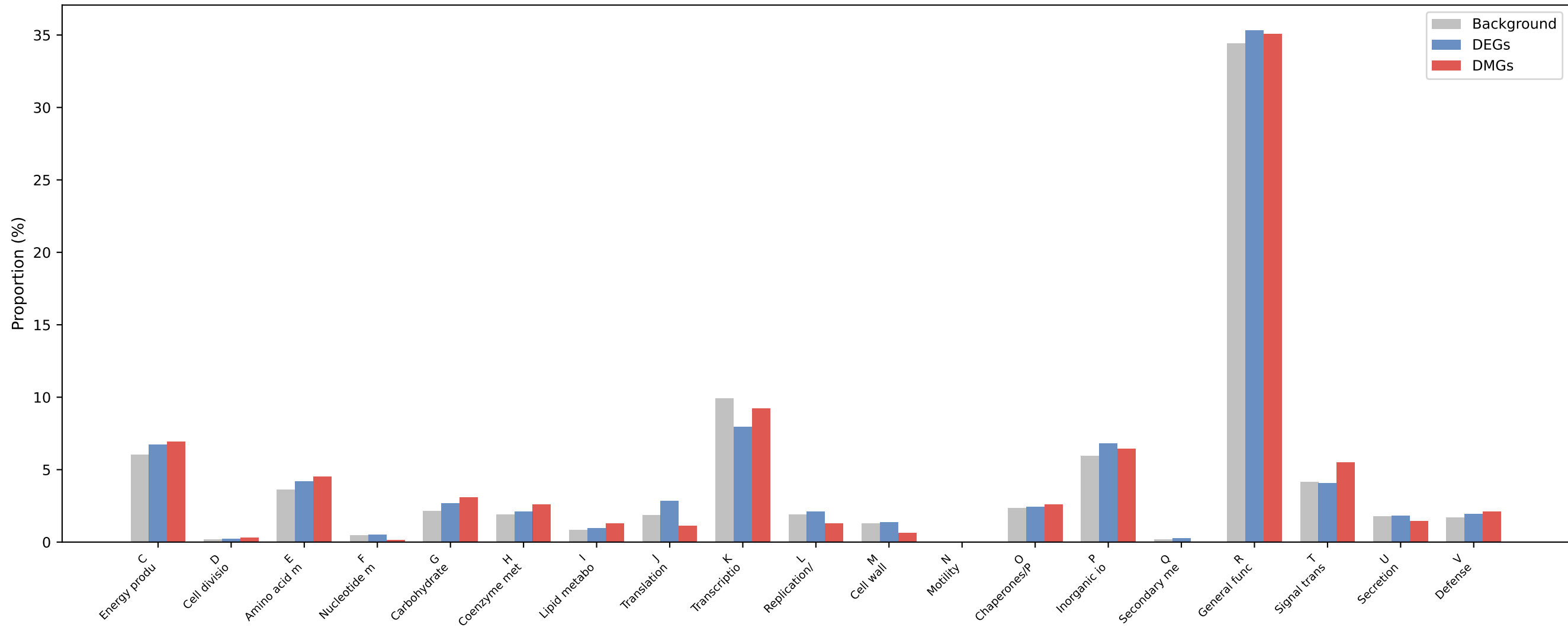
COG Distribution: DMGs vs DEGs vs Background (T3vsT1)
