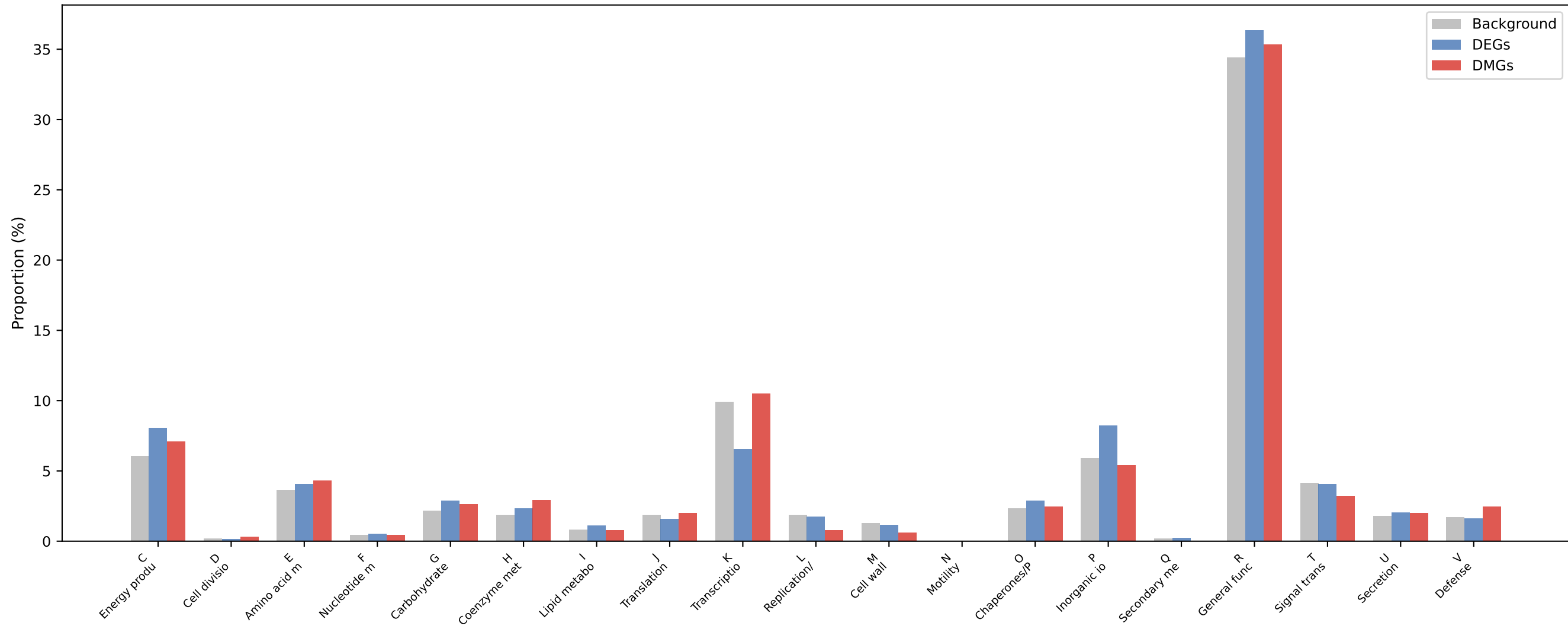
COG Distribution: DMGs vs DEGs vs Background (T3vsT2)
