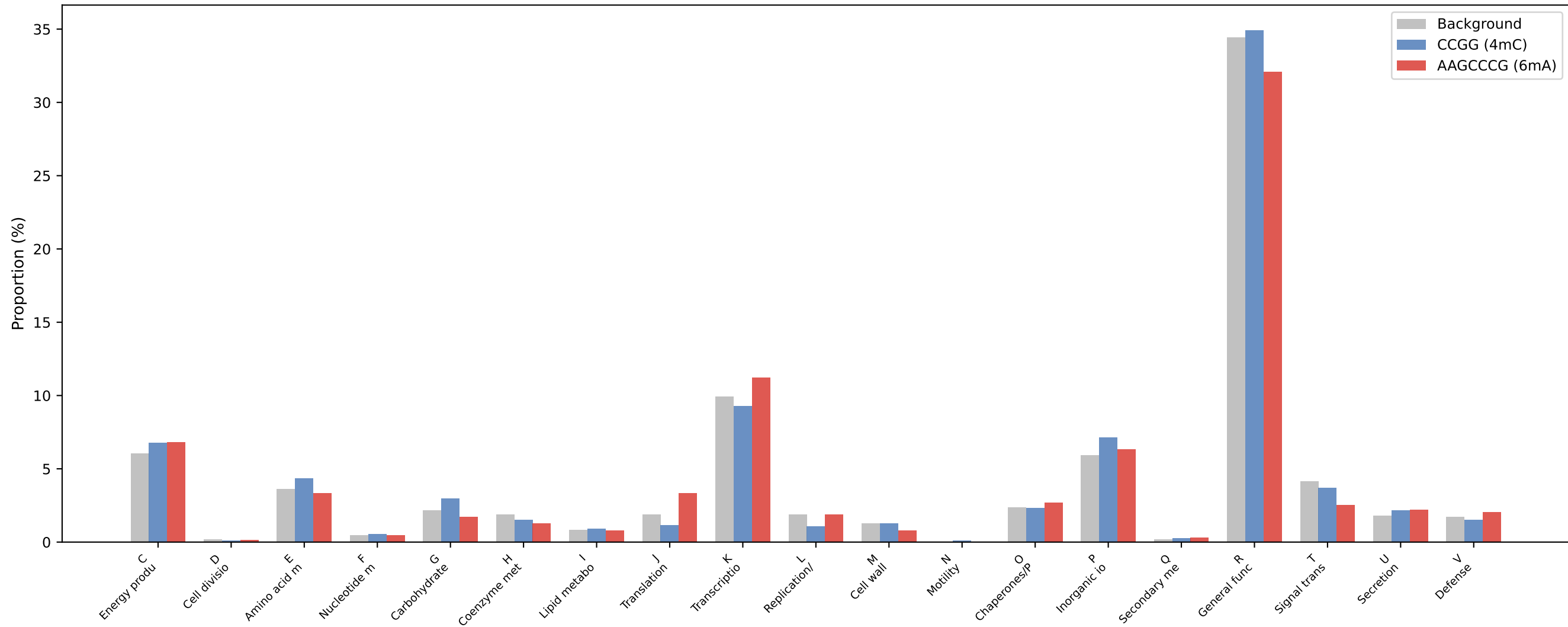
COG Distribution: CCGG vs AAGCCCG Methylated Genes
