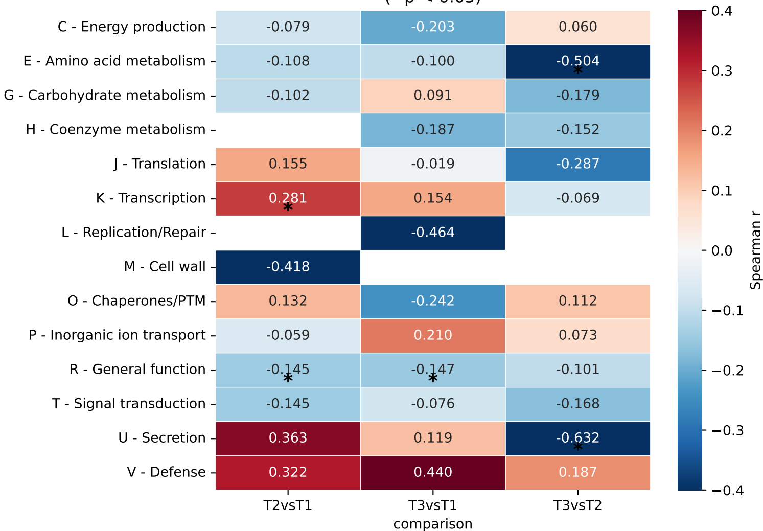
6mA Methylation-Expression Correlation by COG Category (* p < 0.05)
