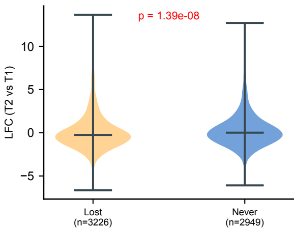
A GCCGGC — Unstratified
