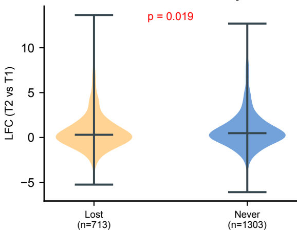
C GCCGGC — Arm only
