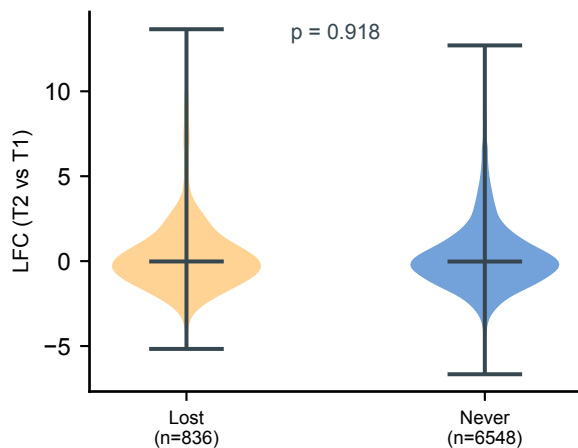
D AAGCCCG — Unstratified
