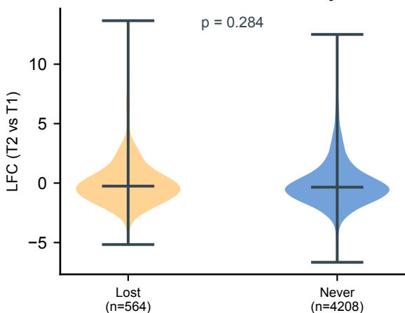
E AAGCCCG — Core only
