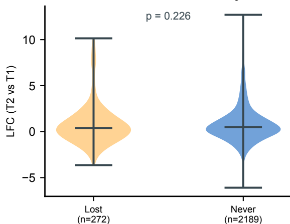
F AAGCCCG — Arm only
