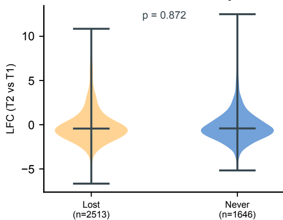
B GCCGGC — Core only
