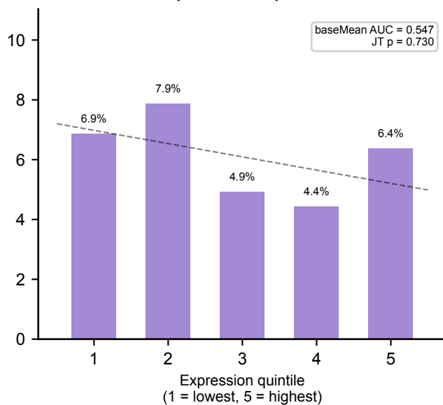
E Expression-independence
