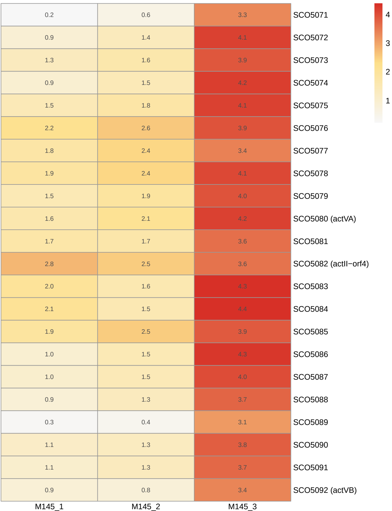
ACT cluster gene expression (log10)
