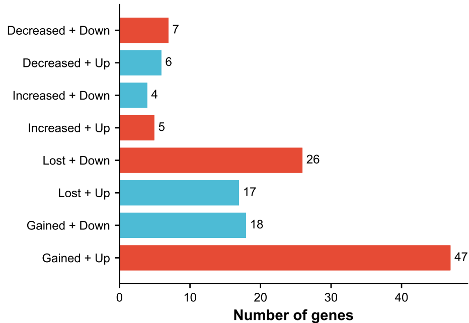
4mC
