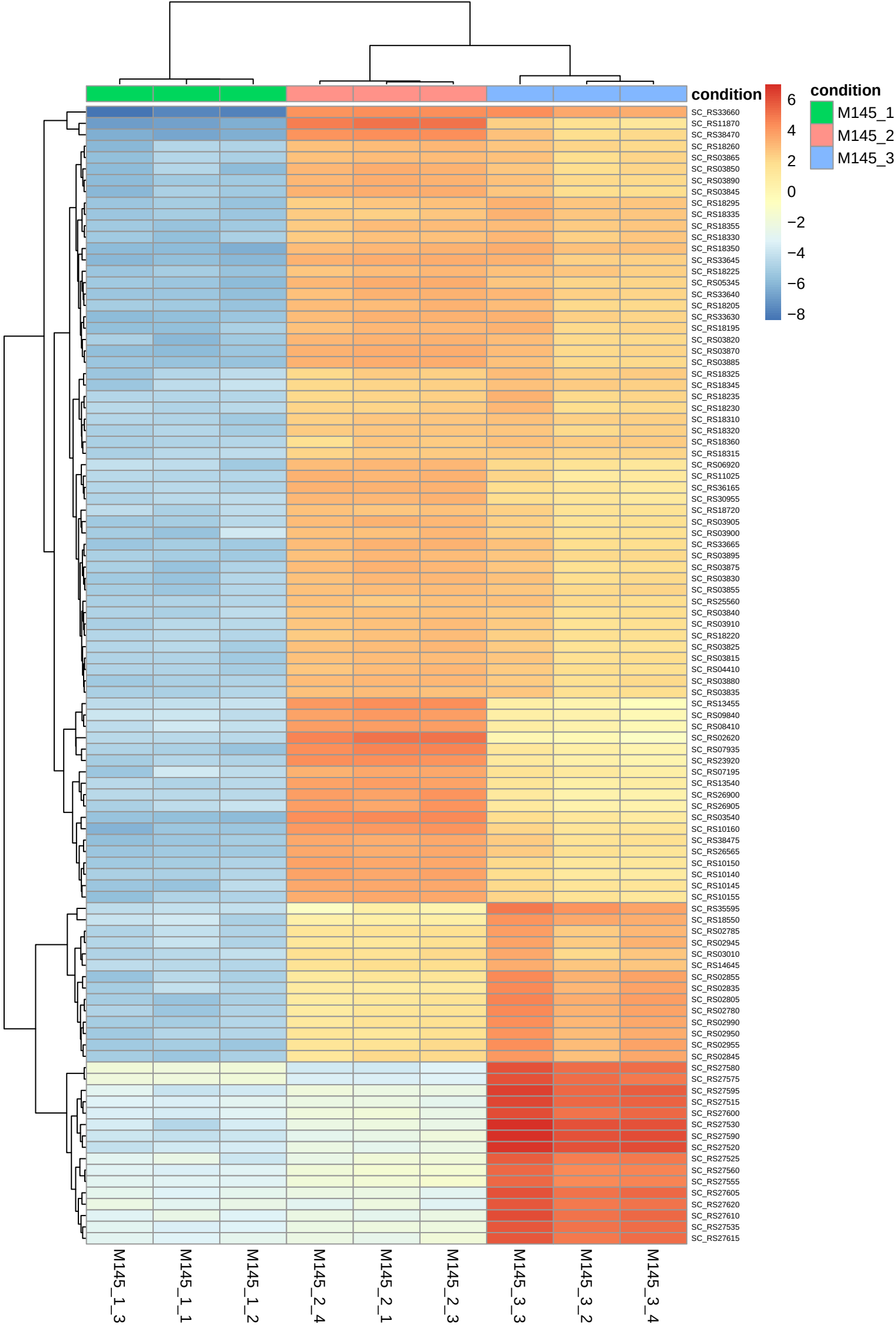
Top 100 variable genes (rlog, row-centered)
