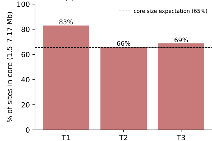
(b) GCCGGC 4mC — core fraction
