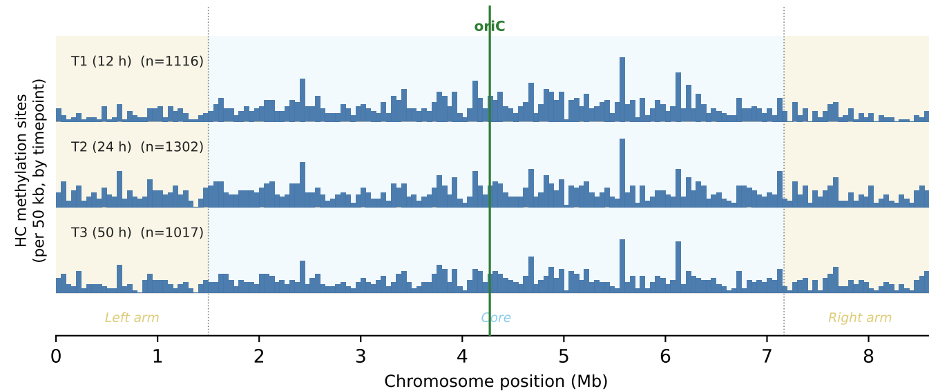
(c) AAGCCCG (4mC + 6mA pooled) — linear chromosome landscape
