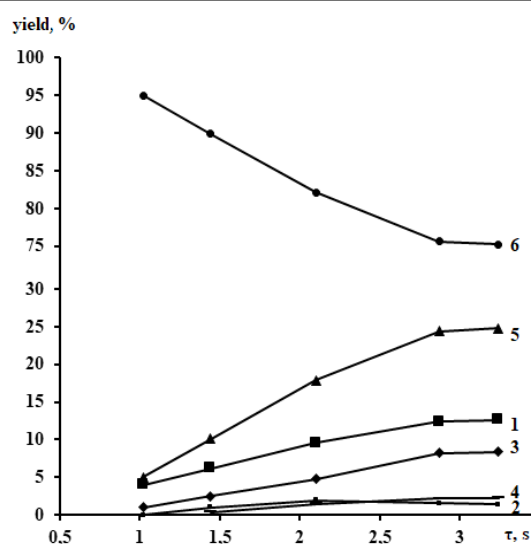
Fig.2. Effect of contact time on the methane monooxidation reaction under the following conditions: tetrakis/ Al_2O_3 ; C_{cat} = 0.64 [mg/g]; t = 300^\circ C ;
