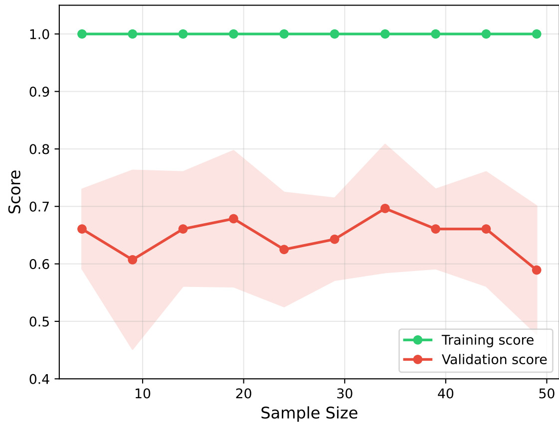
RBF-SVM
