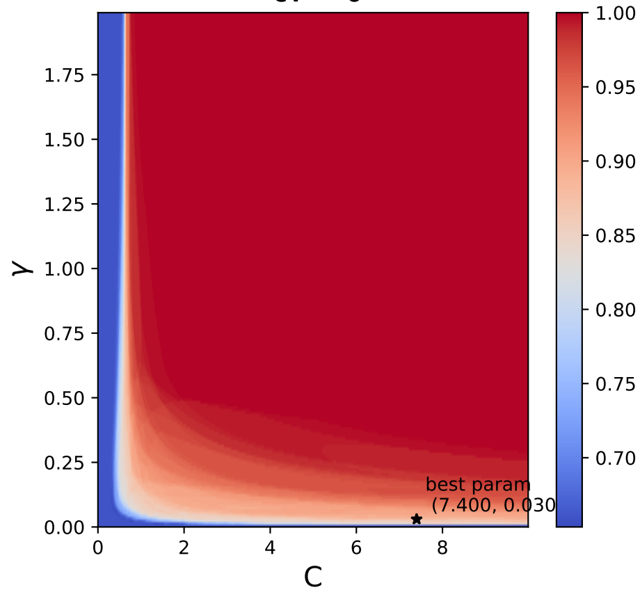
train Accuracy Kernel = rbf cv = 6
