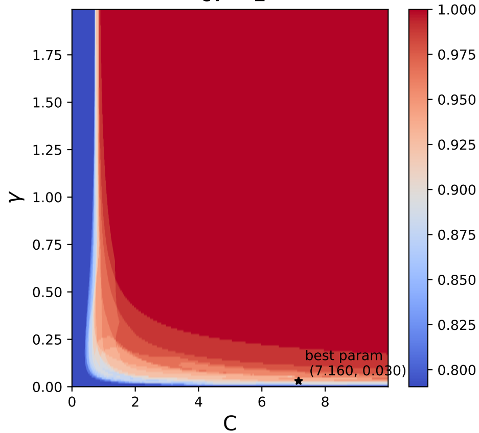
train Accuracy Kernel = rbf cv = 2
