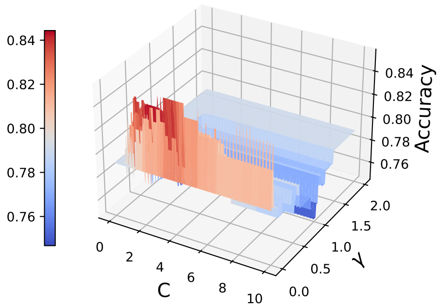
Test Accuracy Kernel = rbf cv = 5
