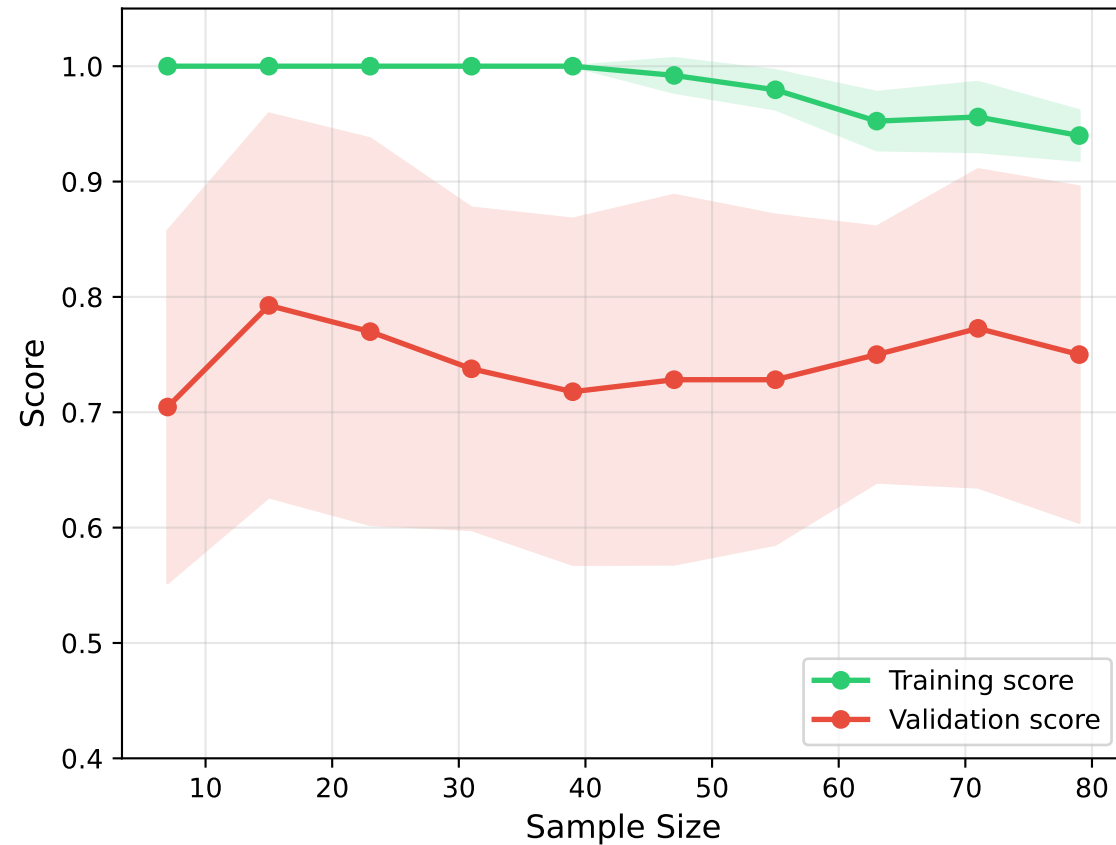
Gradient Boosting
