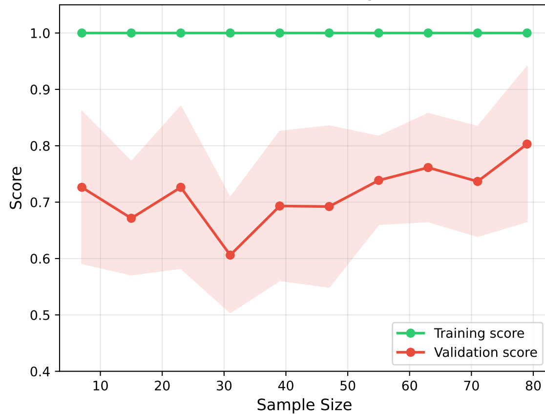
Gradient Boosting
