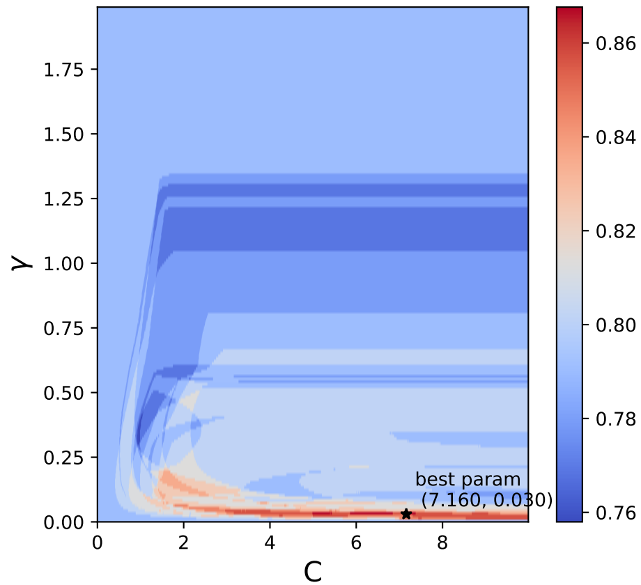
test Accuracy Kernel = rbf cv = 2
