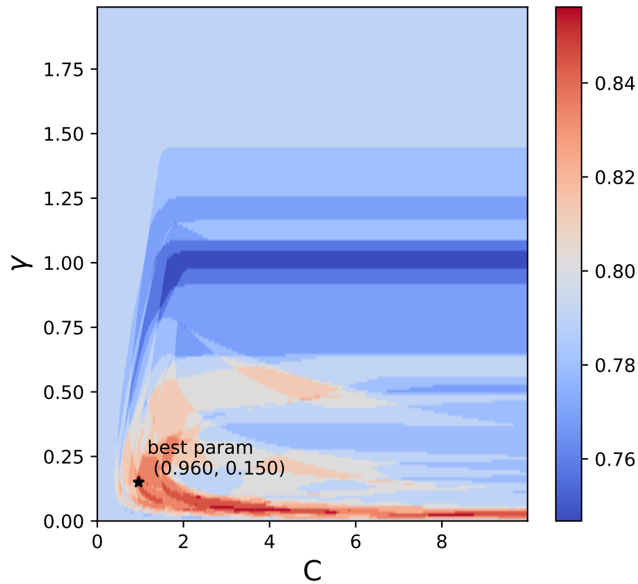
test Accuracy Kernel = rbf cv = 5
