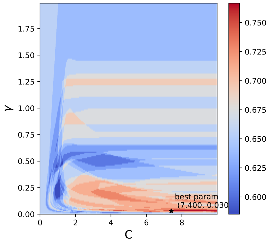
test Accuracy Kernel = rbf cv = 6
