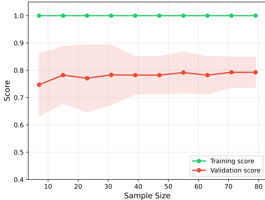
RBF-SVM
