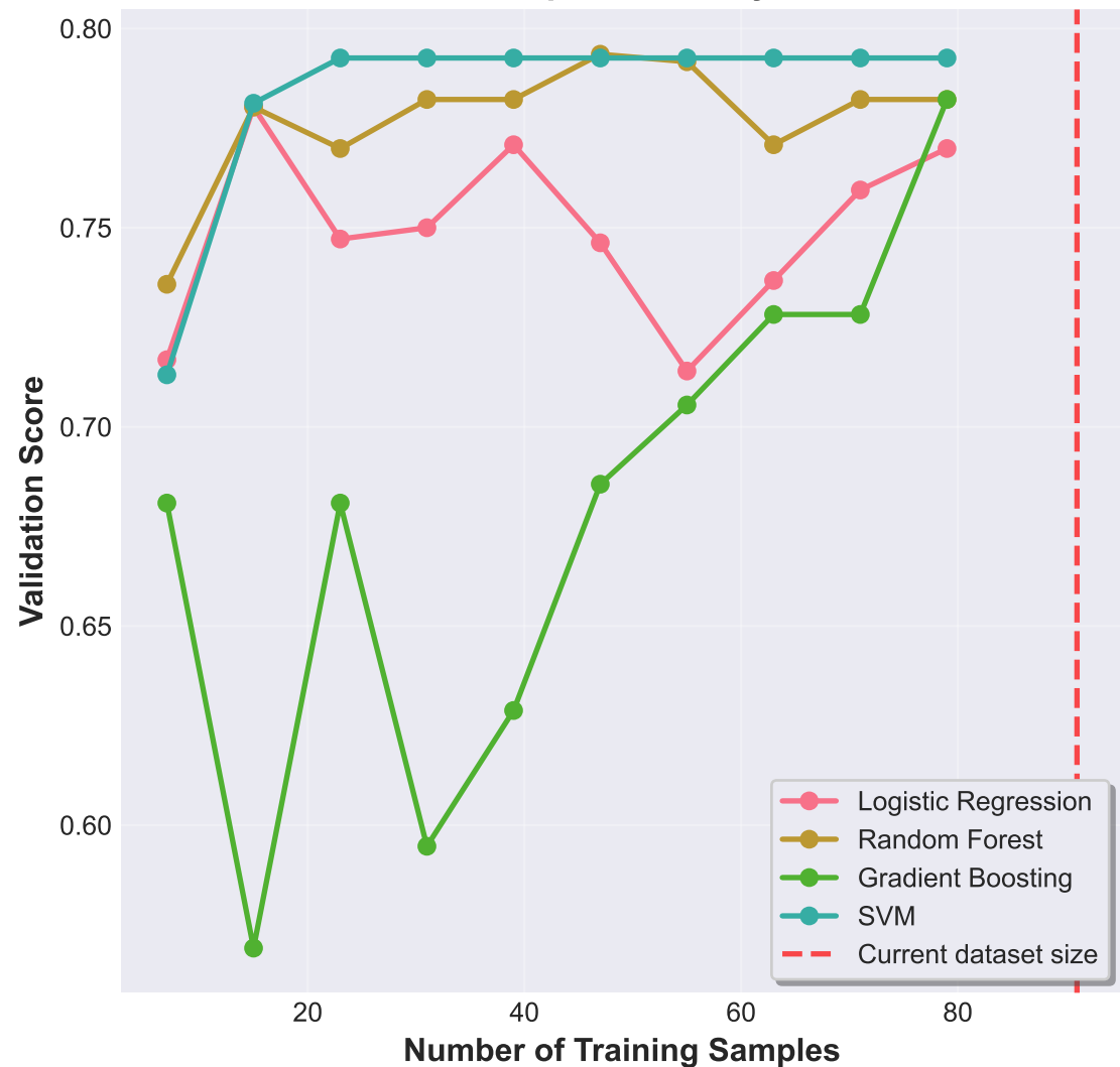
Sample Efficiency
