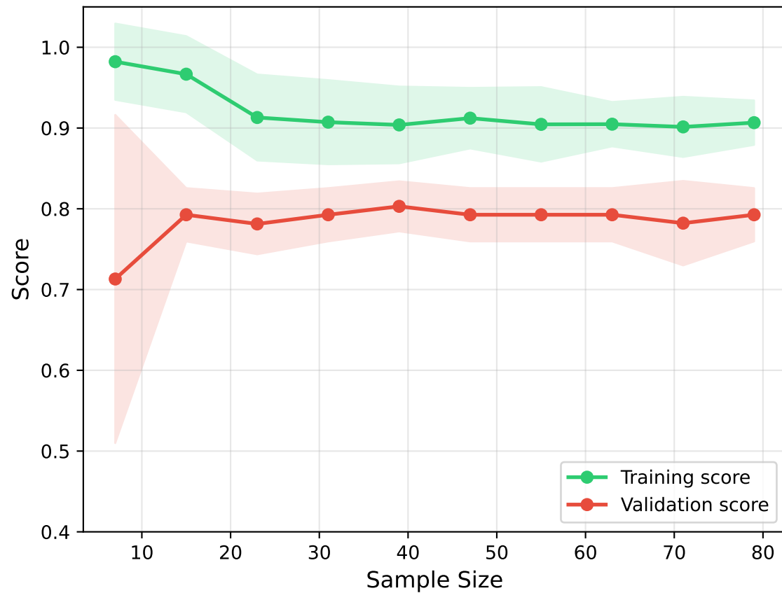
RBF-SVM
