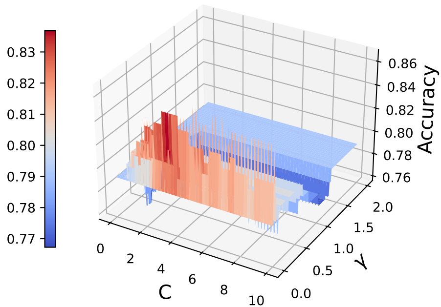
Test Accuracy Kernel = rbf cv = 2
