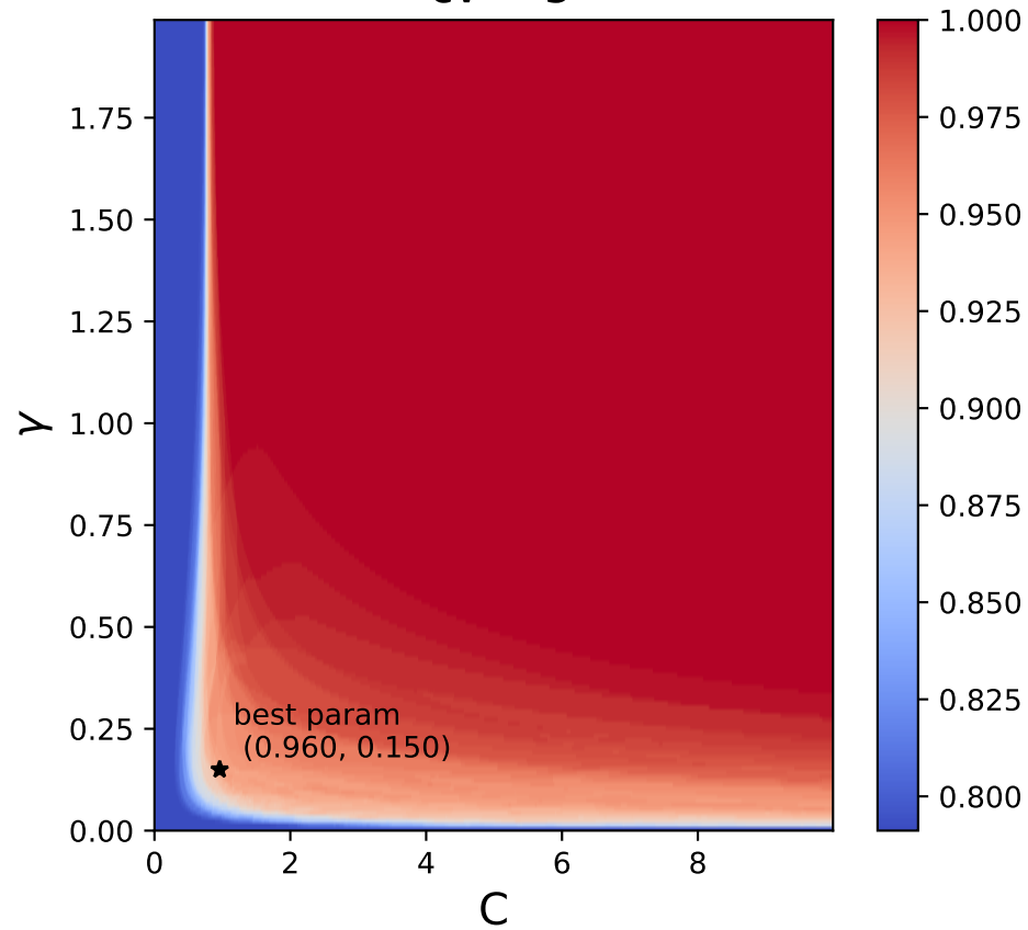
train Accuracy Kernel = rbf cv = 5
