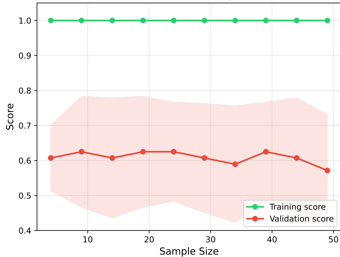
Gradient Boosting
