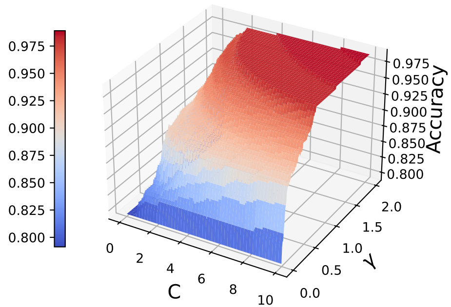
Train Accuracy Kernel = rbf cv = 4
