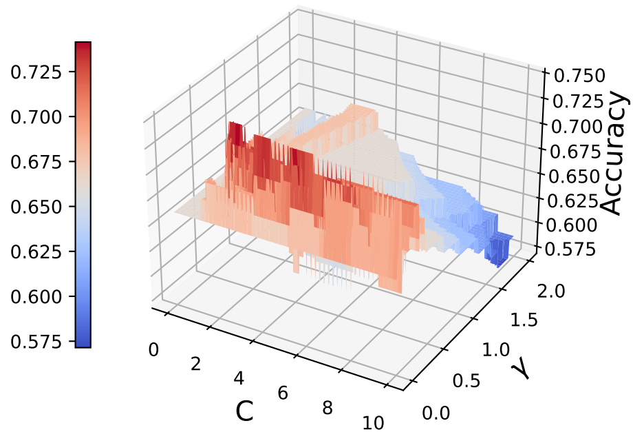
Test Accuracy Kernel = rbf cv = 4
