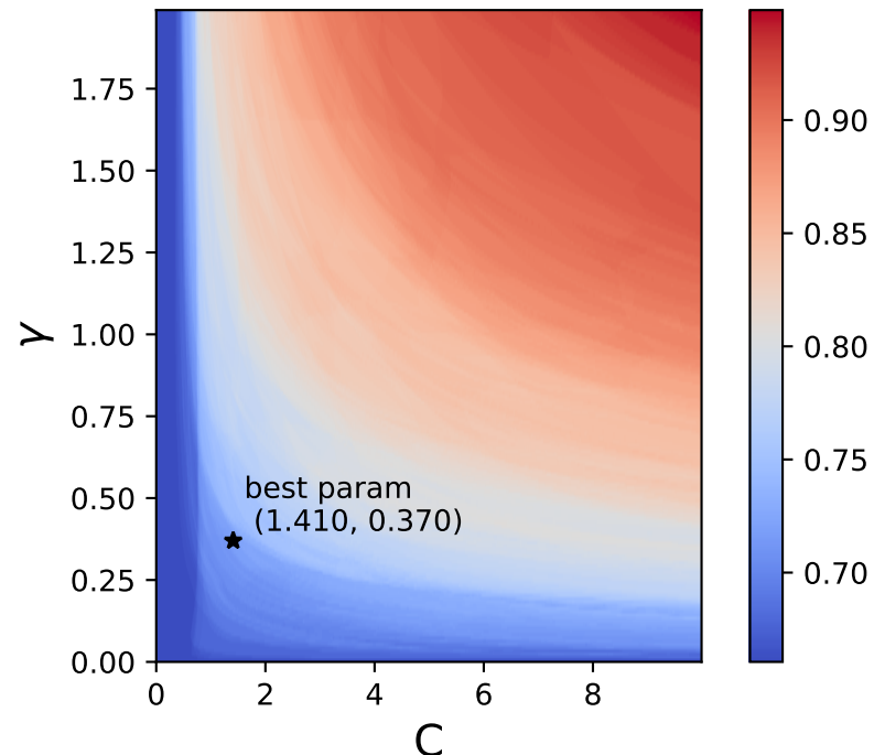
Kernel = rbf cv = 6
