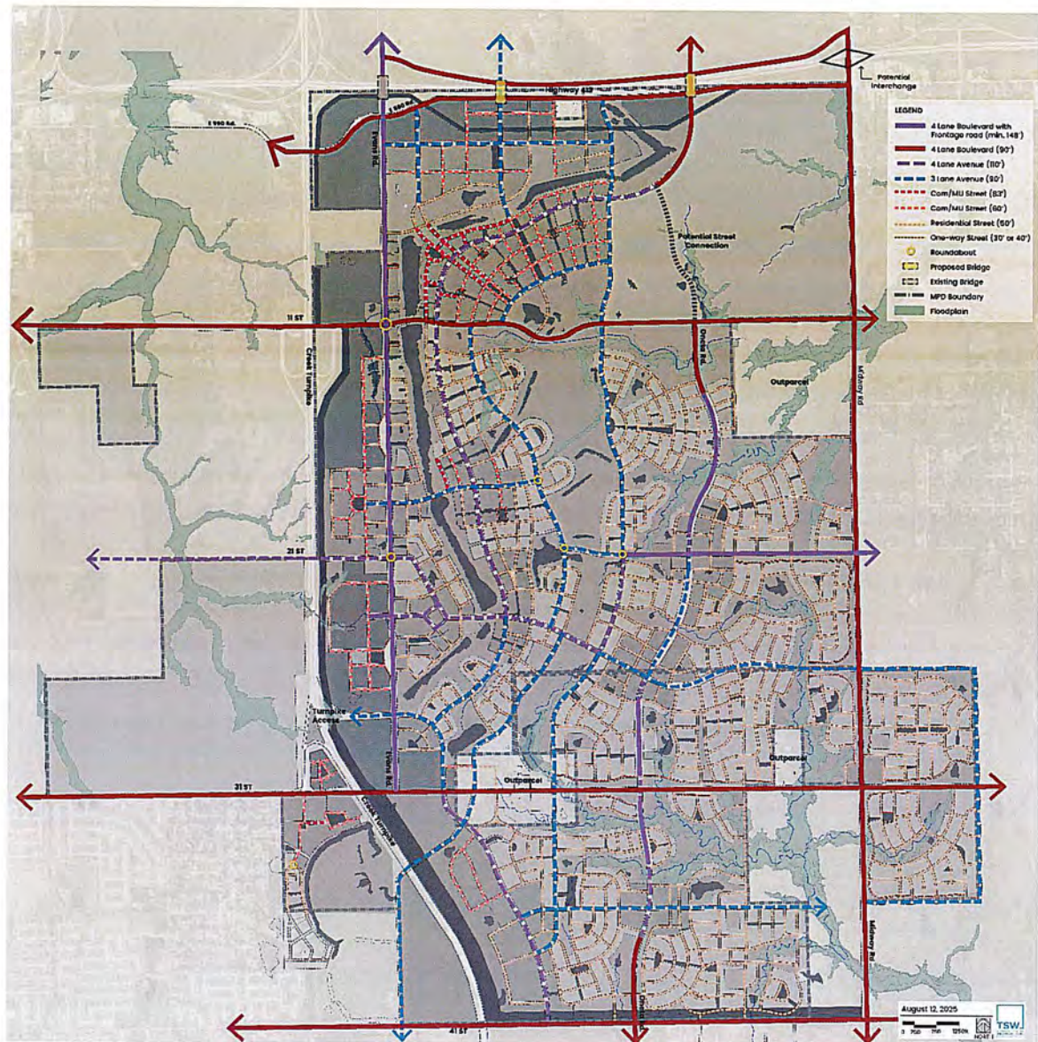
Exhibit 4. Street Network Plan
