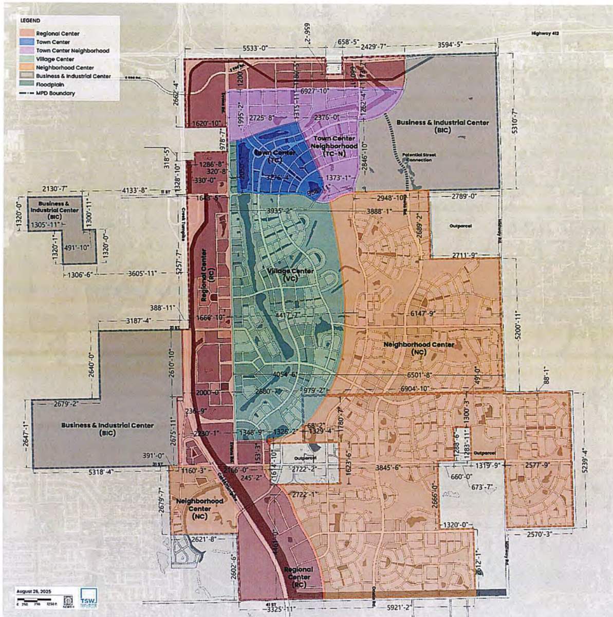
Exhibit 3b. Development Area Plan with Dimensions
