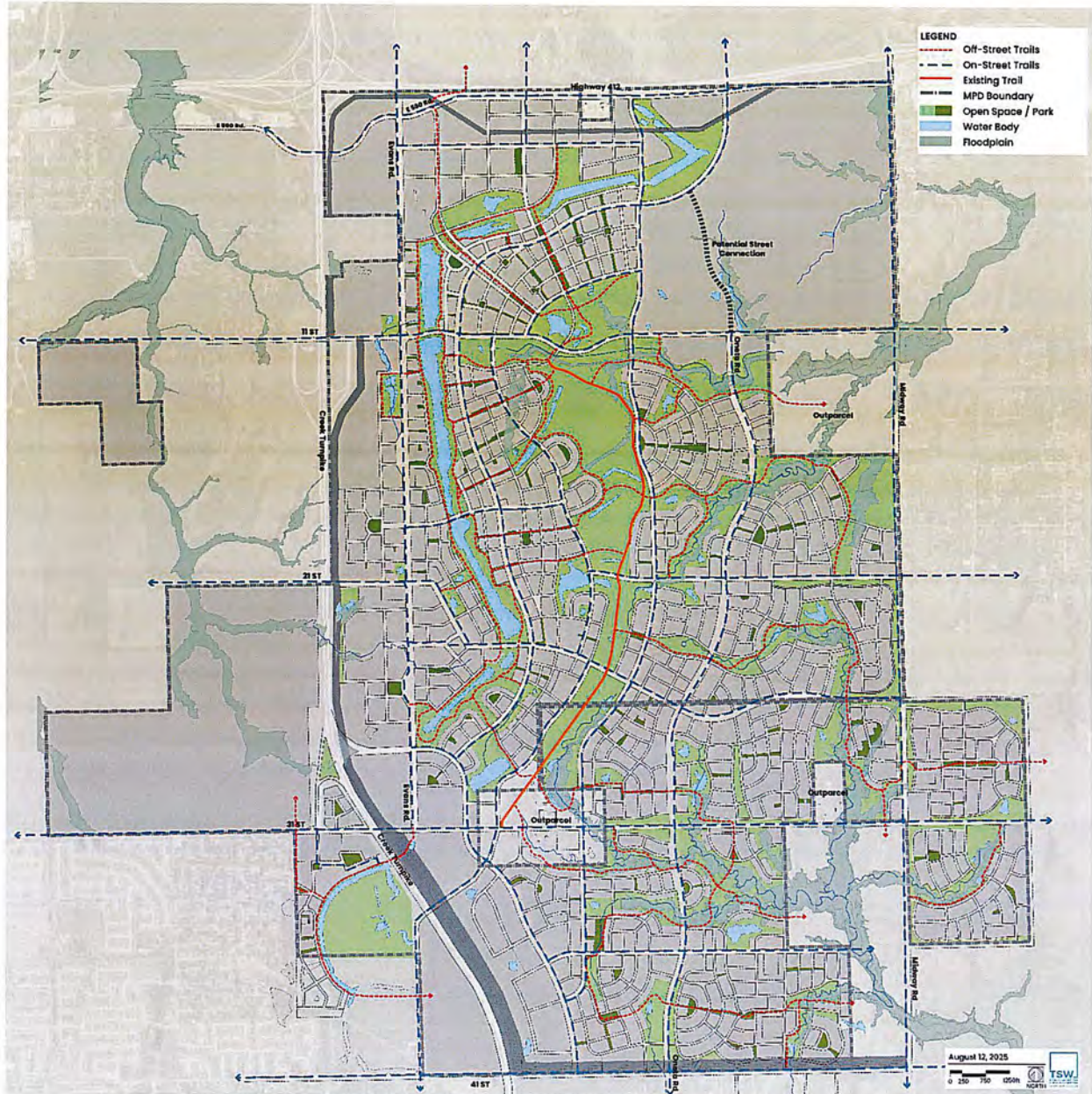
Exhibit 5. Open Space and Mobility Plan
