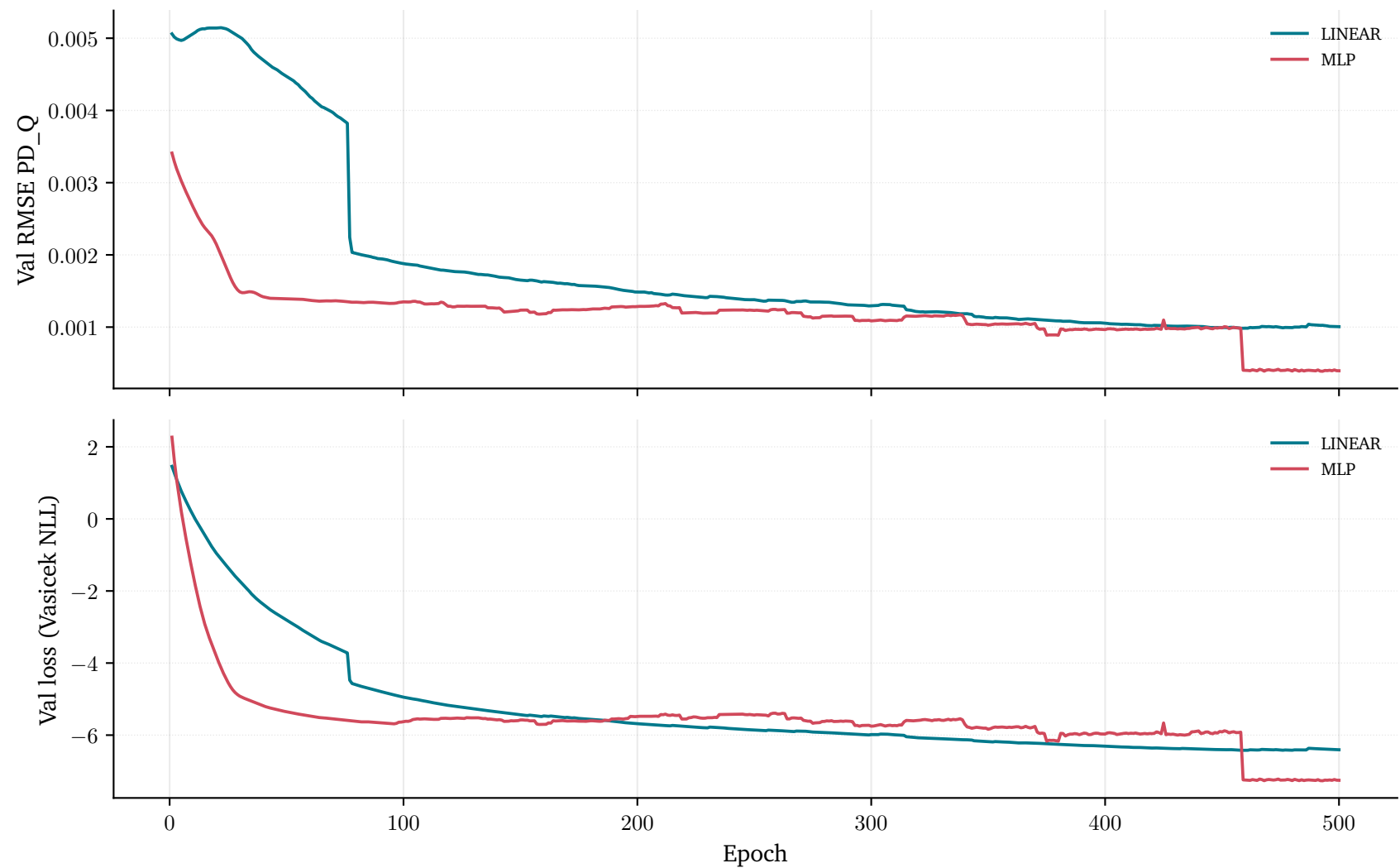
Expanding-window learning curves
