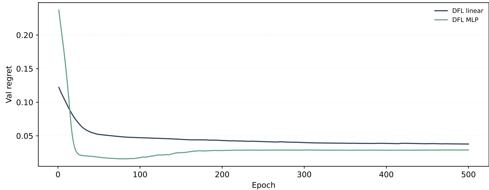
Expanding-window learning curves
