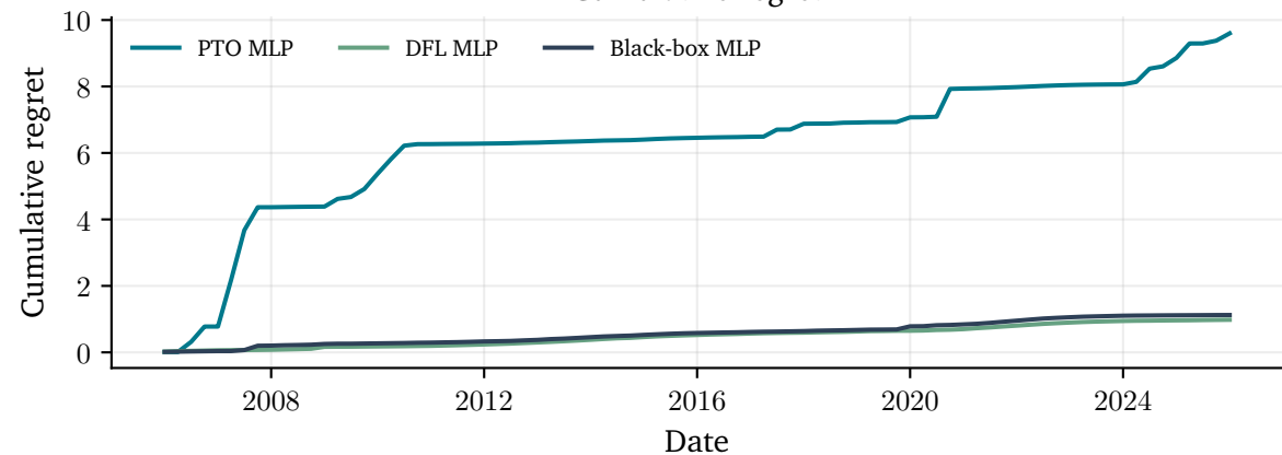
Cumulative regret
