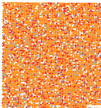
Visium · human breast tumor
