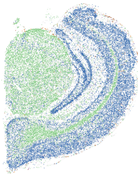
Stereo-seq · adult mouse brain
