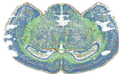
Allen MERFISH · mouse brain
