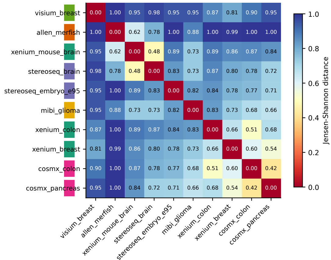
Edge-type composition distance, 10 datasets (clustered)
