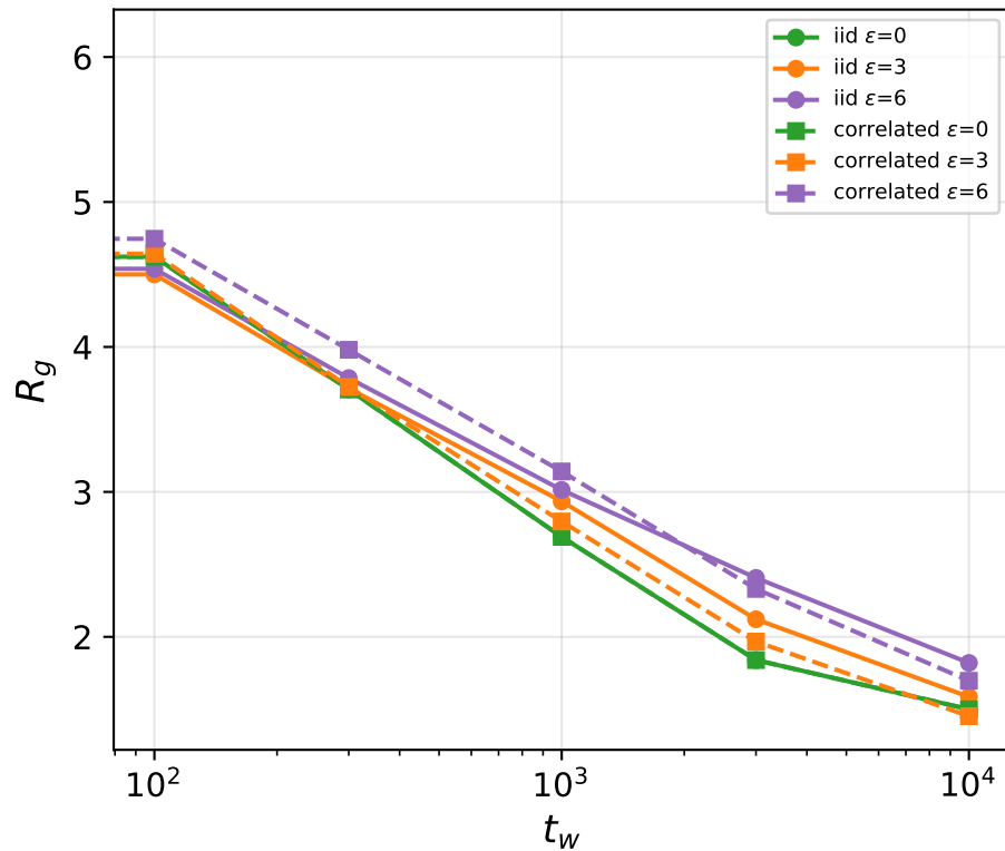
Radius of gyration
