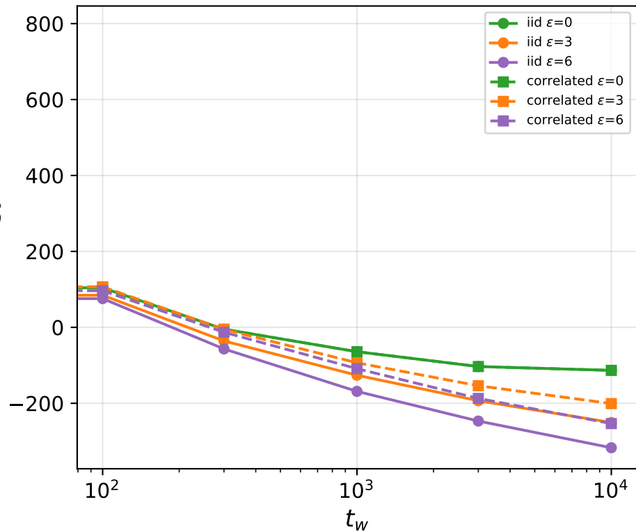
Energy at snapshot
