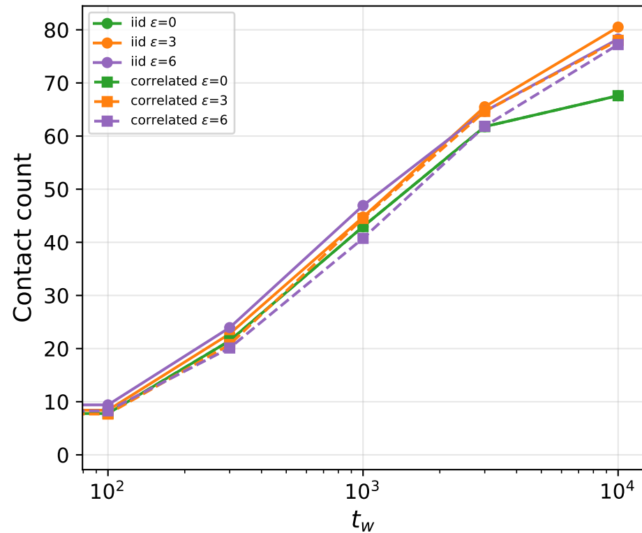
Number of contacts
