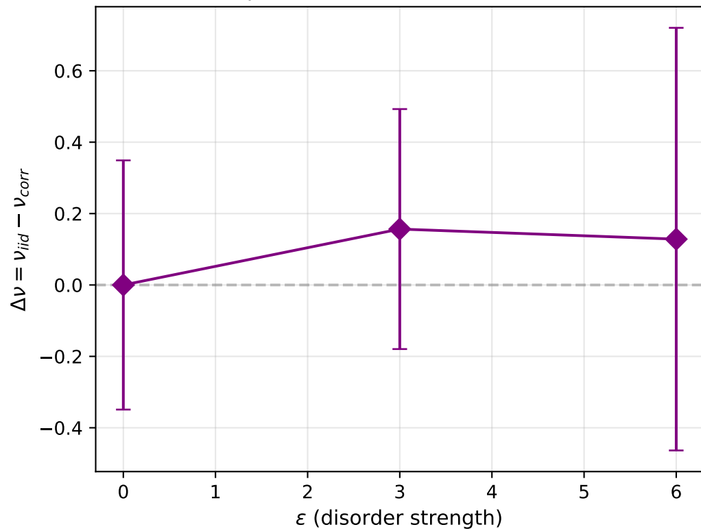
Exponent difference with 95% CI
