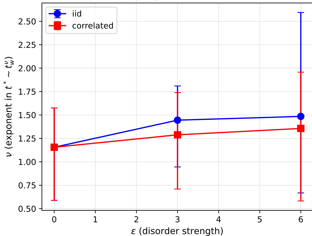
Scaling exponent with 95% CI
