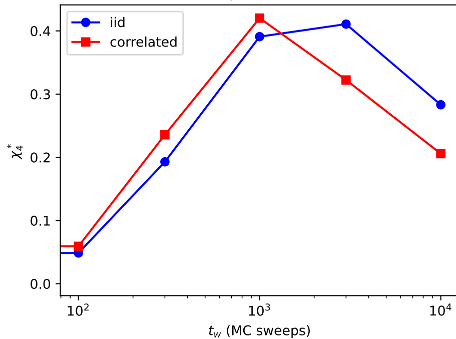
epsilon=3
