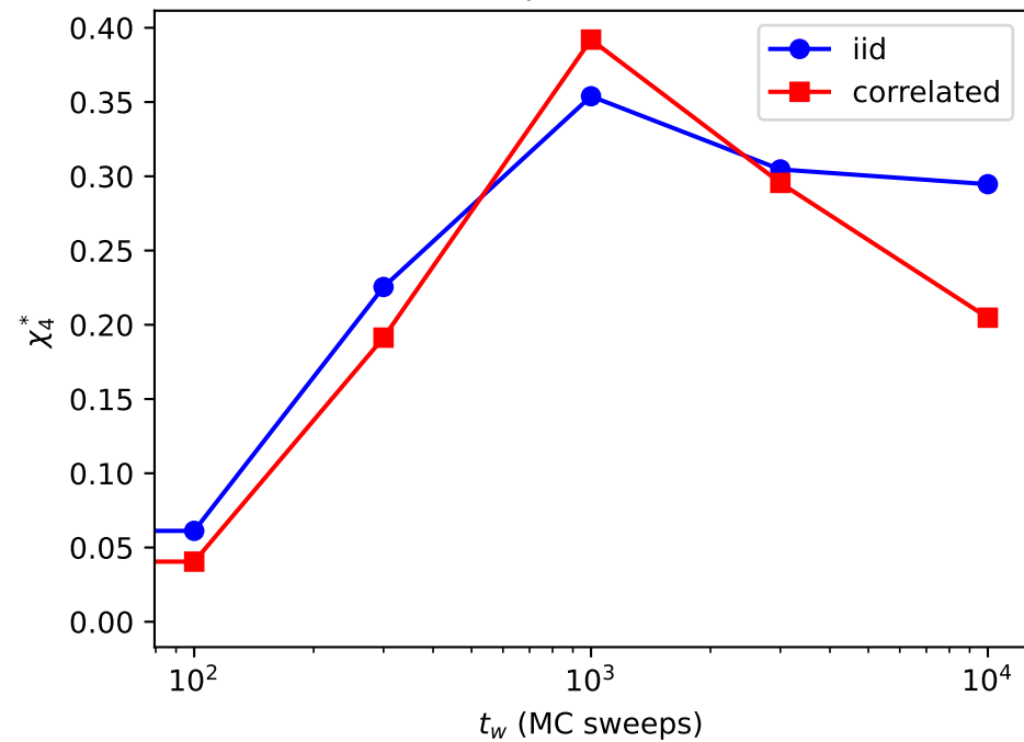
epsilon=6
