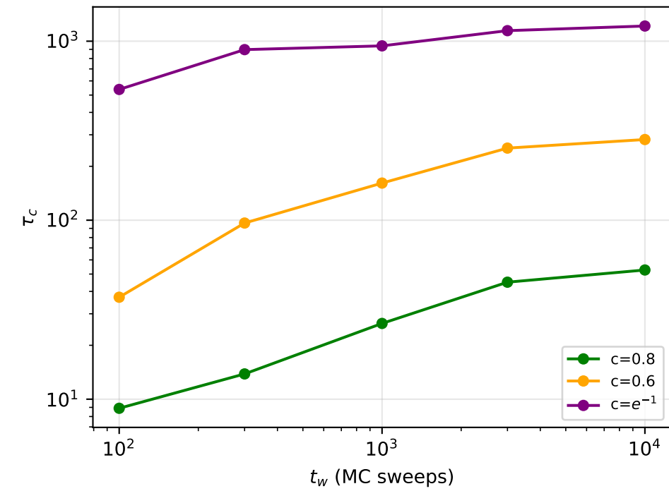
correlated, \varepsilon=0.0
