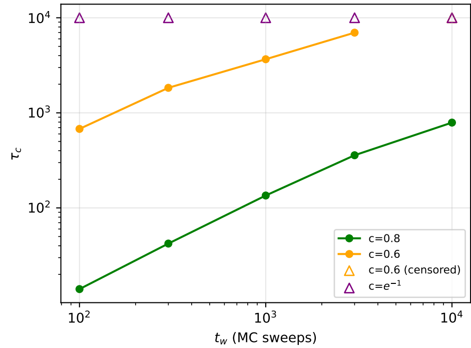
correlated, \varepsilon=6.0
