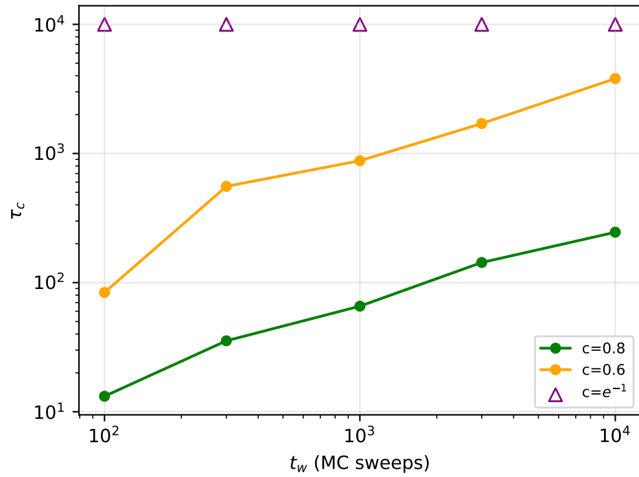
correlated, \varepsilon=3.0
