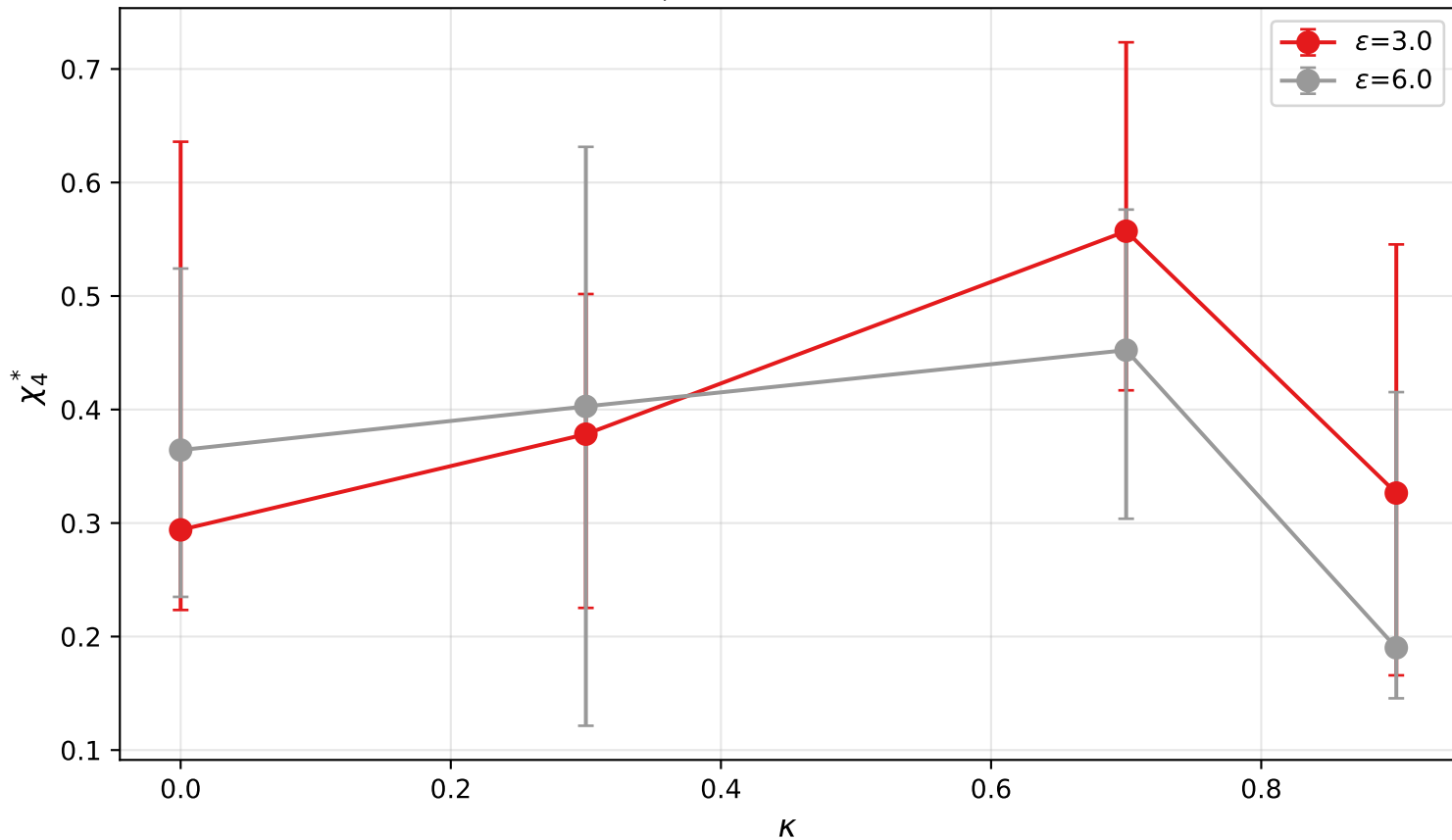
\chi_4^* vs \kappa at t_w=1000
