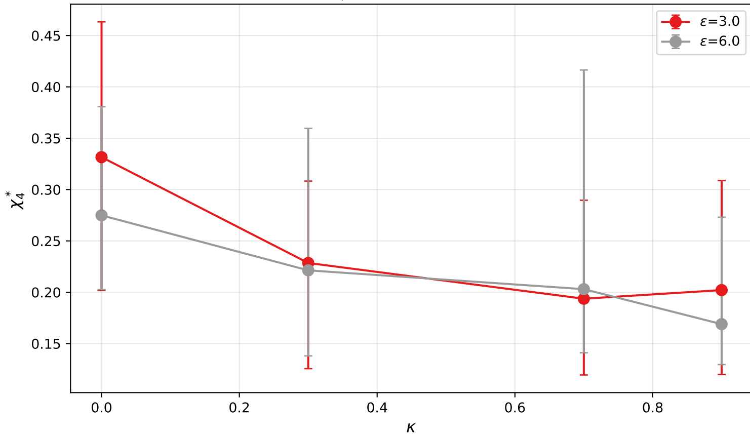
\chi_4^* vs \kappa at t_w=10000
