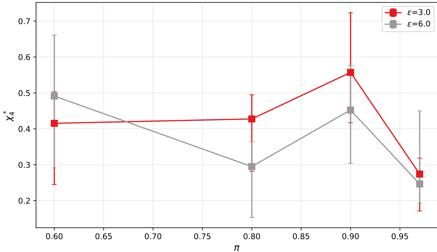
\chi_4^* vs \pi at t_w=1000
