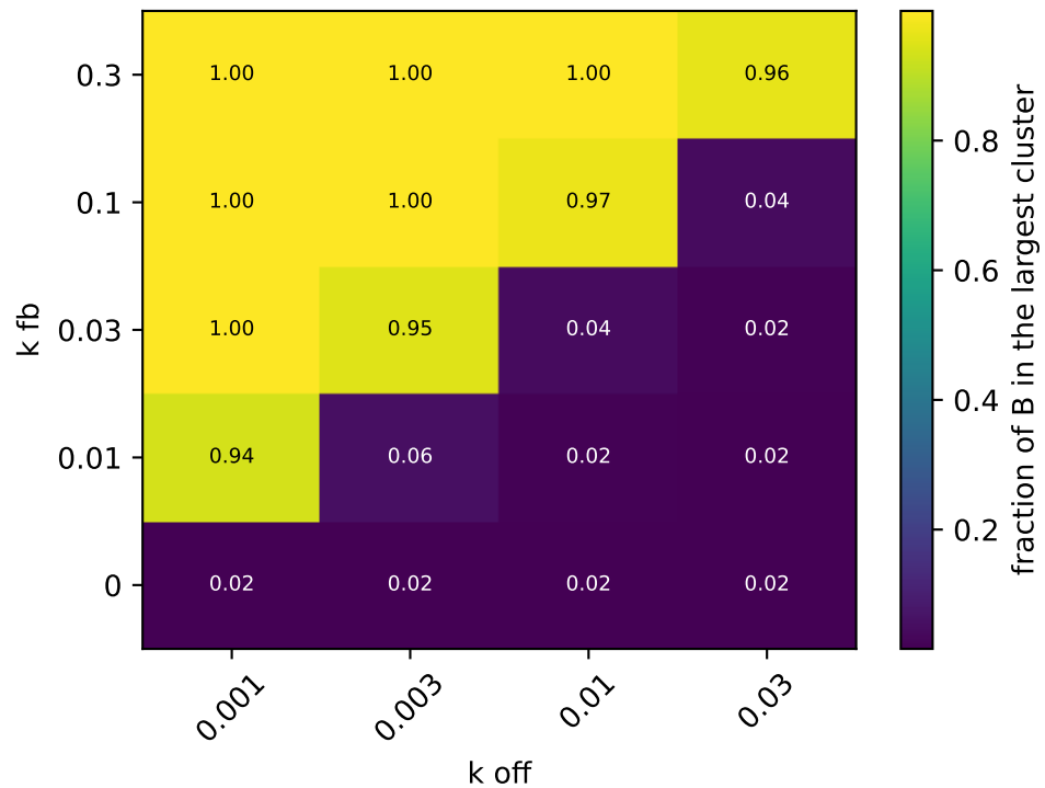
eps_BB=1, f_A=0.7
