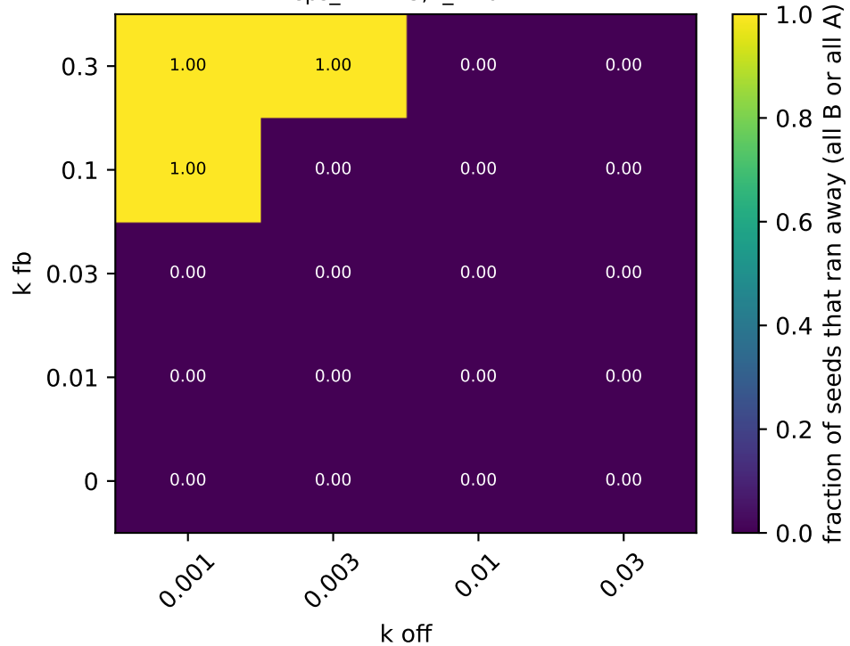
eps_BB=1.5, f_A=0.7
