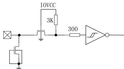
Figure 3-2 Reset Input Port Circuits
