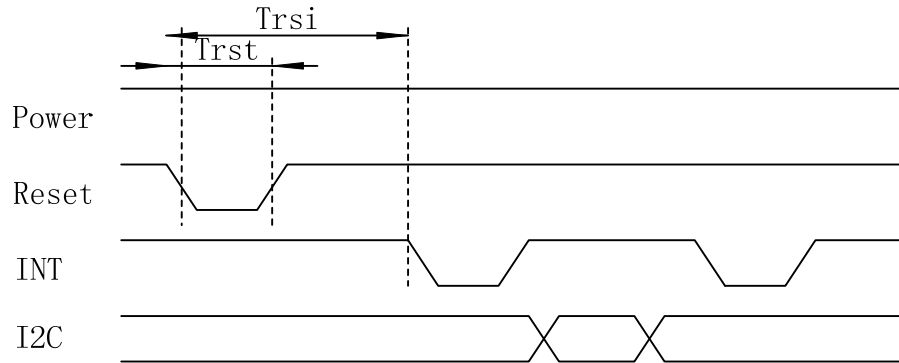
Figure 3-10 Reset Sequence
