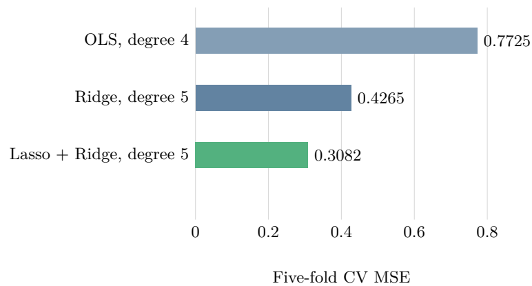
Figure 1. var1: Lasso term selection followed by Ridge reduces validation error.
