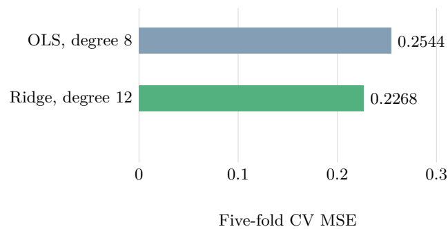
Figure 2. var2: degree-12 Ridge improves on ordinary least squares.
