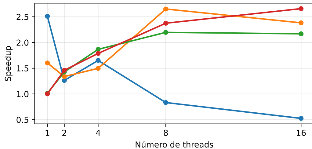
Pthreads
