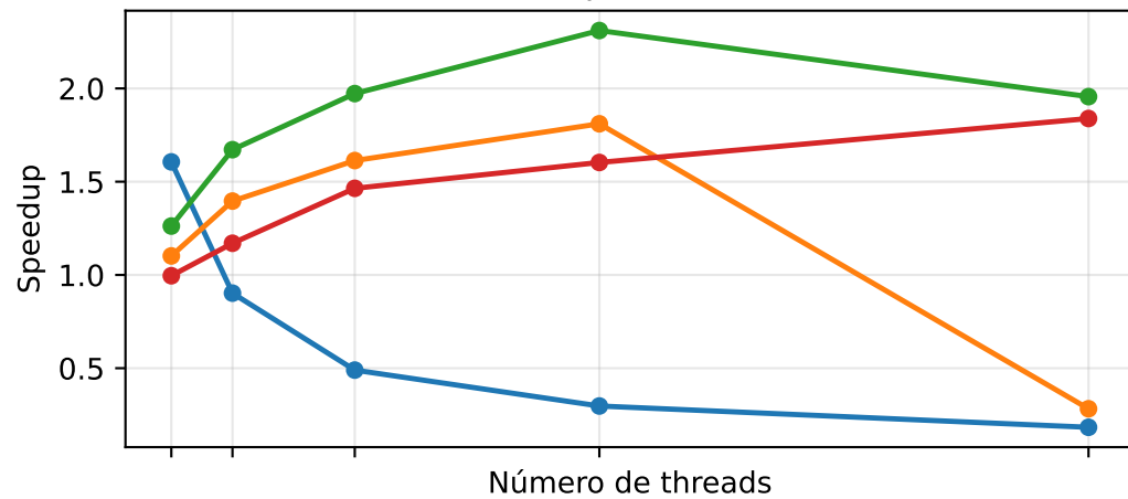
Pthreads
