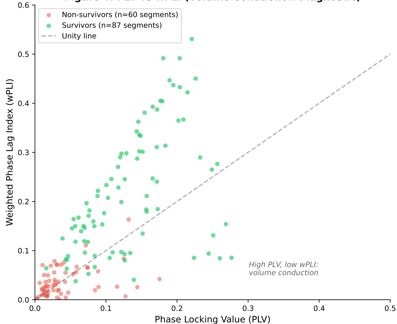
Figure 4: PLV vs wPLI (Volume Conduction Diagnostic)
