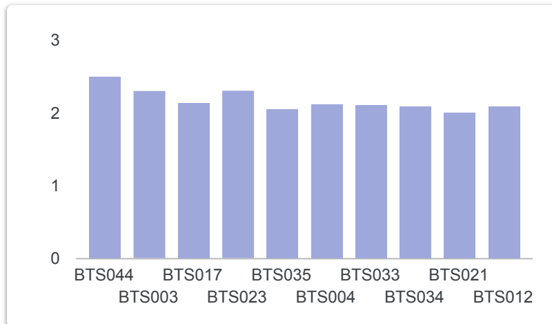
Average Packet Loss by Tower
