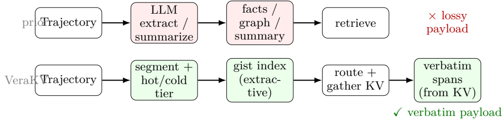
Figure 1: Prior memory systems construct a lossy store (extract/summarize/ graph) and retrieve from it. VeraKV keeps raw segments, builds only a cheap extractive gist index over the cold ones, and at query time routes to and gathers the selected spans’ KV verbatim—gist routes, verbatim answers.
