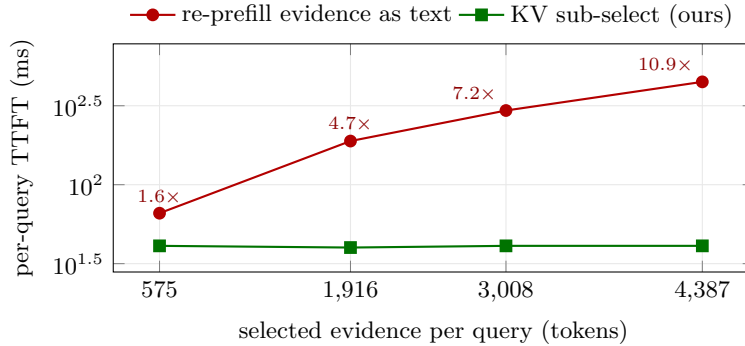
Figure 4: KV sub-selection decouples per-query latency from evidence size. As a query selects more evidence, re-encoding it as text grows TTFT (66 → 448 ms; dense Qwen3-8B), whereas gathering the selected spans’ KV re-encodes only the question and stays flat (~40 ms); the widening gap is the per-query speedup (labeled, 1.6\times \rightarrow 10.9\times ), reaching 32\times at 32k selected tokens (§4.5). First-token argmax matches the full-encode oracle at every point.
