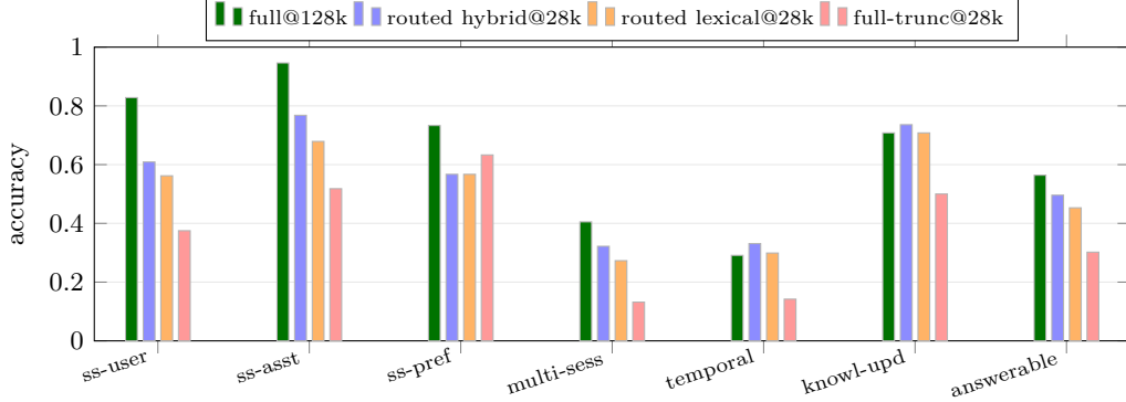
Figure 2: LongMemEval-S per-type accuracy, full 500 questions (Qwen3-32B served at 128k via YaRN; internal Qwen3-32B judge; 95% bootstrap CIs on answerable in §4.3). Two regimes: when the 115k haystack fits the window, full context wins overall (answerable 0.564), but routed selection at 4.5\times less budget leads on temporal and knowledge-update; at a 28k budget where the history must truncate, routed selection (0.496) beats truncation (0.302) by +19 pp, and the embedding-hybrid router beats lexical by +4 pp. Correct-abstention (not shown) is 0.60/0.67/0.67/0.77.
