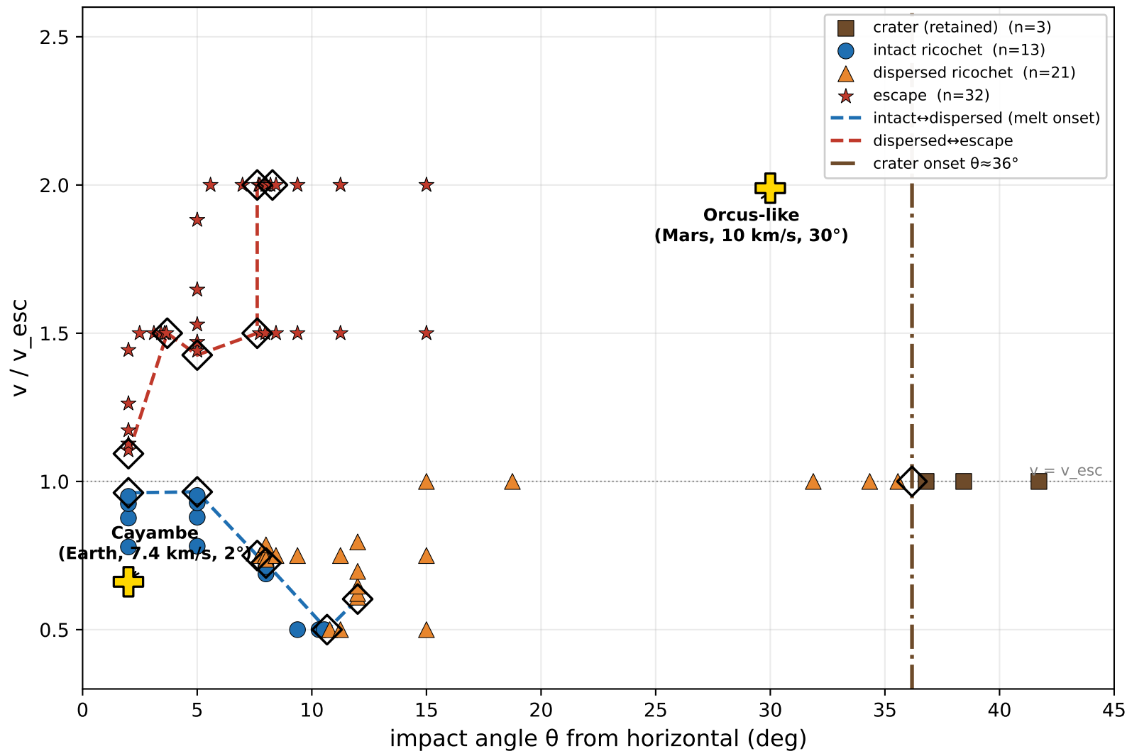
Grazing-impact bounce-off phase diagram — km iron on rock (69 GPU-SPH runs, CPPR=8; 13/13 boundaries bisected)
