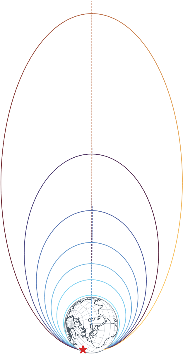
view down the capture-orbit angular momentum (dashed = per-pass apsidal rays; apogee-direction spread 0.7°)
