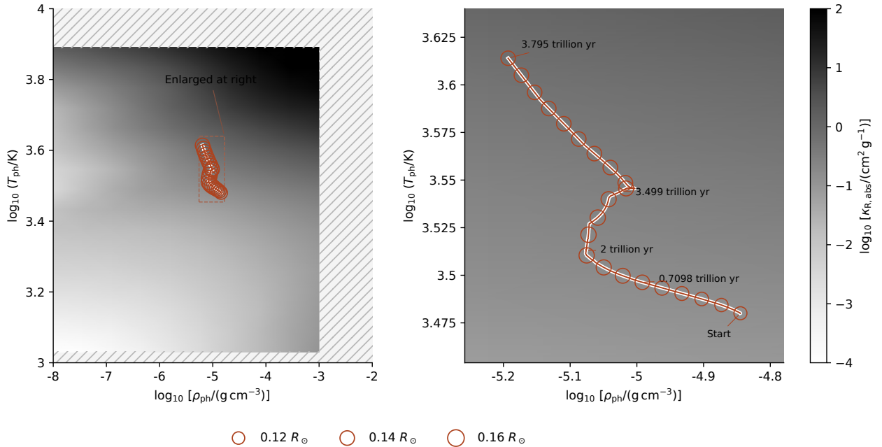
Figure 4: Photospheric progression of the 0.1 M_{\odot} Ember model through 3.795 Tyr, following the layout of LBA97 Figure 6. The line contains all 6836 accepted stellar models; 22 selected models are shown as open circles, with diameters proportional to radius. Labels give the actual saved ages. The right panel enlarges the region visited by Ember. Density and local temperature are interpolated from the gas atmospheres at Rosseland optical depth 2/3, using the evolving surface composition. The grayscale background is a fixed hydrogen-rich reference: the Rosseland absorption mean of the SYNSPEC wavelength table at X = 0.7 , Z = 0.02 and zero {}^3\text{He} . It excludes scattering and grains and does not represent the changing total opacity along the track. LBA97’s background includes grain opacity, producing a band of high opacity at low temperature that is absent from this gas-only map. Their figure also spans several stellar masses and includes contraction and cooling; here only the calculated hydrogen-burning track is shown. Hatching marks conditions outside the plotted opacity table.
