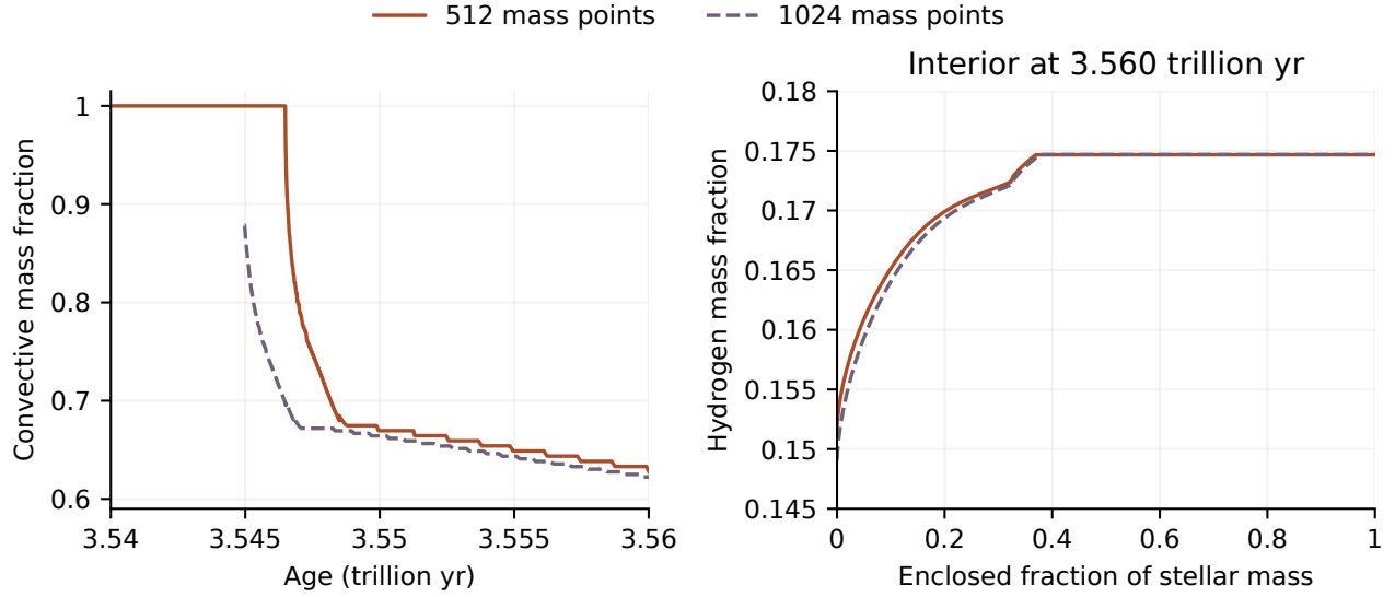
Figure 3: The change from full convection, compared at two mass resolutions. Left: the fraction of stellar mass in convective regions falls sharply near 3.545Tyr and continues declining. The 1024-point history shown starts at its saved restart; the earlier part of that curve is not reconstructed. Right: hydrogen profiles at 3.560Tyr. Both centers are now stable against convection, while the outer convective region retains a nearly uniform hydrogen fraction. The difference between central abundances is visible despite close agreement at the surface. The curves retain every saved value.
