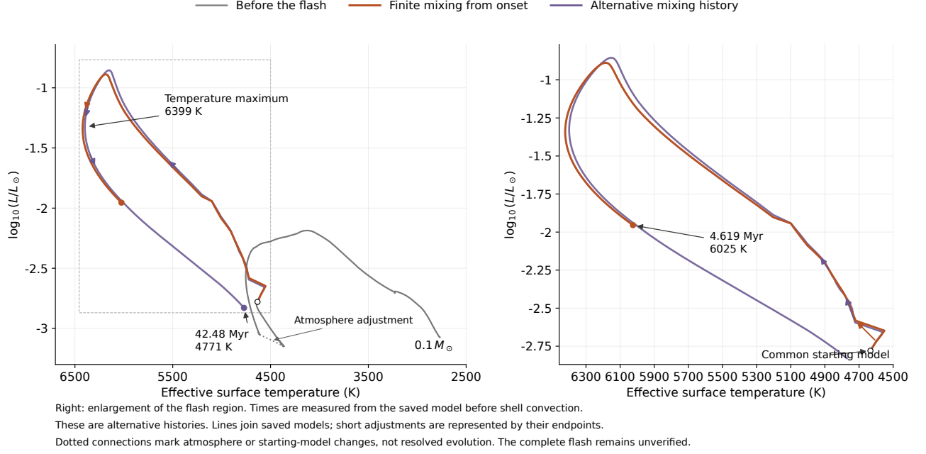
Figure 6: The two computed histories through helium-3 burning and subsequent contraction. Orange follows finite convective mixing from the onset of shell convection; purple follows the alternative mixing history. Their endpoints are 4.619 Myr at 6025 K and 42.48 Myr at 4771 K, respectively. Times are measured from their common model before shell convection. The right panel enlarges the flash region. Gray shows the preceding evolution; dotted connections indicate atmosphere or starting-model adjustments rather than resolved evolution. Agreement in the HR diagram does not establish convergence of the flash’s peak power or internal mixing.
