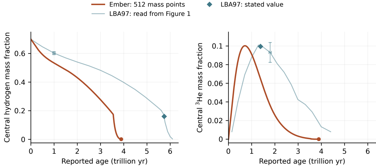
Figure 14: Hydrogen consumption and the buildup and depletion of ^3\text{He} in the pp comparison without microscopic separation. The pale curves are read from the inset of LBA97 Figure 1, with 20 hydrogen and 15 helium-3 samples. Diamonds show their stated ^3\text{He} maximum and the hydrogen abundance at central radiative-core formation. Orange curves are the 512-point Ember track through 3.890Tyr. Ages are shown as reported, without shifting or stretching either calculation. The representative crosses correspond to four image pixels: about 0.05Tyr in age and 0.01 in mass fraction. They illustrate reading precision, not statistical or physical uncertainty. The rapid final hydrogen decline is poorly resolved in the printed inset; the helium-3 trace ends as it becomes indistinguishable from the baseline.
