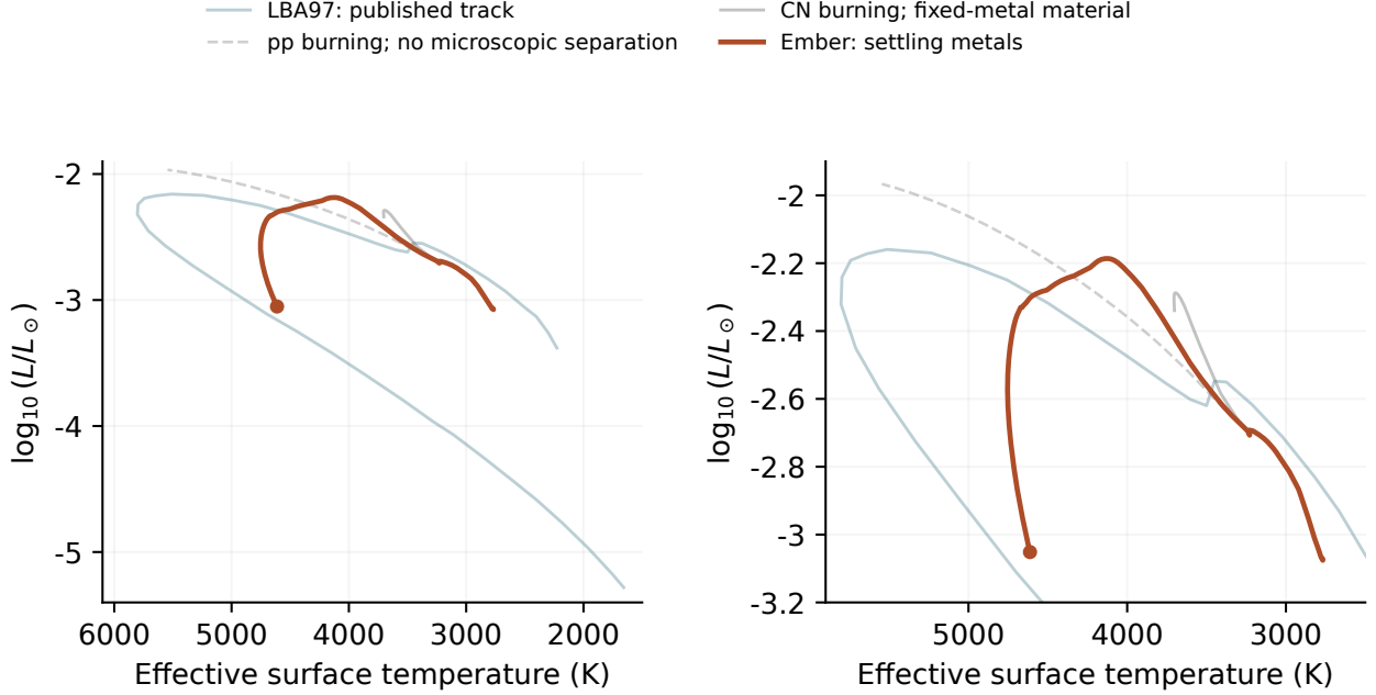
Figure 13: HR diagrams showing the calculation with metal settling through 4.002Tyr (orange), the fixed-metal CN/diffusion comparison through 3.704Tyr (solid gray), the pp comparison without microscopic separation through 3.890Tyr (dashed gray), and LBA97 (pale blue). The left panel shows the wider range and the right panel the hydrogen-burning portion. The orange curve uses the same accepted states as Figure 1.
