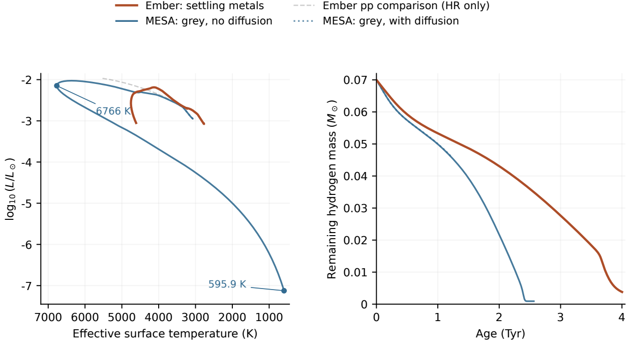
Figure 11: Ember and independent MESA calculations at 0.1M_{\odot} . The left panel includes the computed grey MESA cooling branch; the right shows the remaining total hydrogen mass. Solid blue denotes MESA without diffusion; dotted blue denotes the same grey calculation with diffusion, through 1.225 Tyr. Orange is the same Ember trajectory as Figure 1. The faint dashed grey HR curve is Ember’s pp comparison without microscopic separation. The MESA curves shown here use grey atmospheres, not the separate tabulated-atmosphere configuration. MESA ages include contraction, whereas Ember ages start at its static hydrogen-burning model. The MESA contraction phase preceding the common starting model is omitted from these curves.
