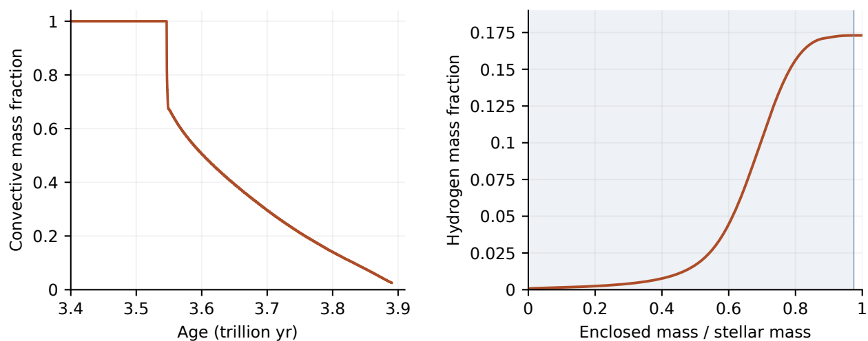
Figure 15: Convection and chemical separation by nuclear burning and macroscopic mixing in the pp comparison without microscopic separation. Left: the fraction of mass in convective regions declines from unity near 3.546Tyr to 0.02565 at 3.890Tyr. Right: the hydrogen profile in the 3.890Tyr model. The shaded core carries heat by radiation and conduction; the outer convective envelope has an almost uniform hydrogen abundance. Both panels use the same calculation and its final saved structure.
