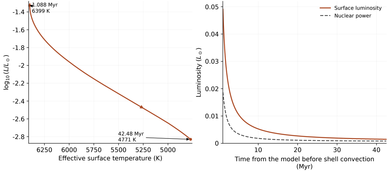
Figure 7: The late shell-burning calculation on 2115 mass points. Left: an enlarged HR diagram around the effective-temperature maximum. The arrow follows increasing time. Right: photon luminosity and deposited nuclear power over the same interval. Time is measured from the model before shell convection. Temperature declines from 6399 K to 4771 K over 4.139 \times 10^7 yr; nuclear burning supplies 55.85% of the final surface luminosity. The contracting model has turned toward cooling. Its physical connection to the calculation resolving the flash from its onset remains unverified.
