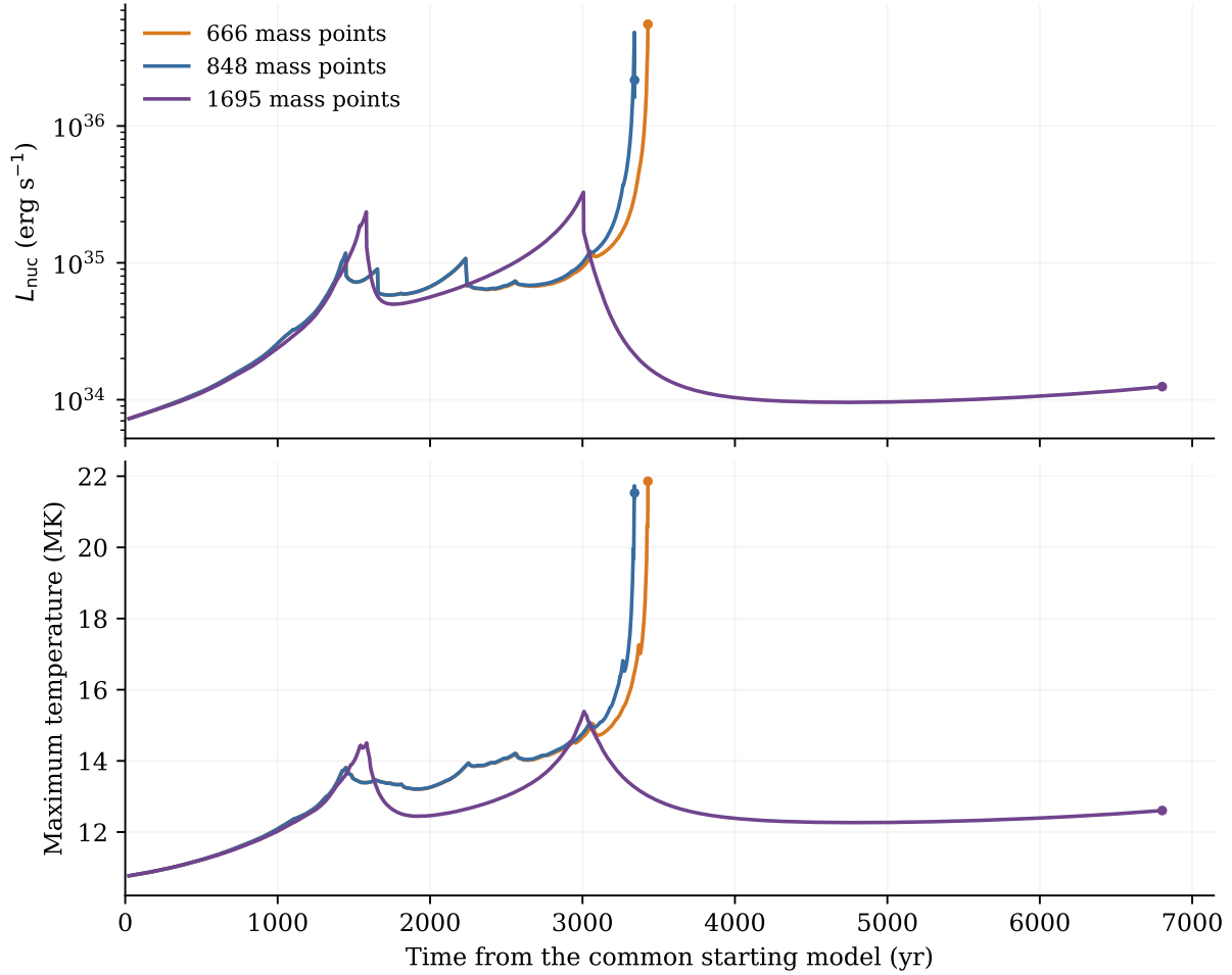
Figure 7: Nuclear luminosity and maximum internal temperature with total energy and composition enthalpy transported across the same mass surfaces. The three grids start from the same underlying stellar profile; adding points requires a small mechanical readjustment. All use the supplied white-dwarf atmosphere and finite convective mixing, with no semiconvective mixing. Time is measured from the common profile before shell convection. The 666- and 848-point endpoints reach 21.86 and 21.53 MK, respectively. The finest grid reaches 12.60 MK after a long decline and modest reheating. Sharp decreases near 3006 and 3341 yr accompany convective-region mergers. Different endpoints reflect the intervals computed so far. The full pulse amplitude, subsequent cooling and atmosphere sensitivity remain undetermined.
