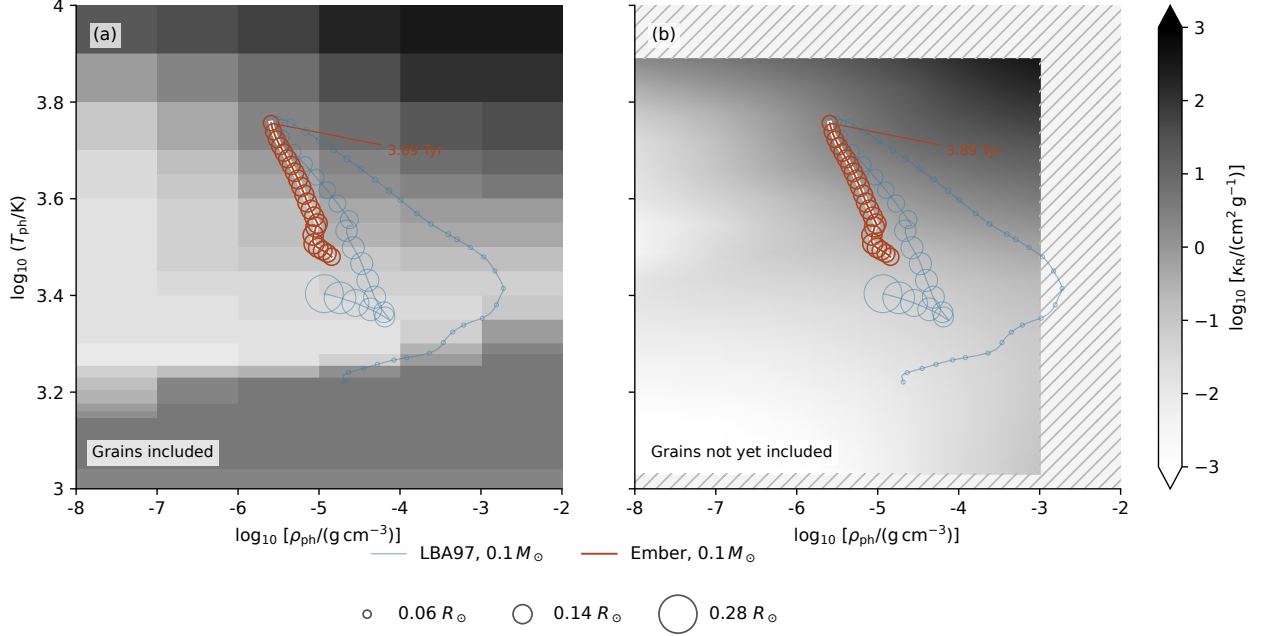
Figure 15: Photospheric evolution of the 0.1M_{\odot} pp comparison without microscopic separation, over hydrogen-rich opacity maps: (a) the grain-inclusive LBA97 Figure 6 map on an approximate calibrated opacity scale; (b) the Rosseland absorption mean of Ember’s SYNSPEC wavelength table at X = 0.7 , Z = 0.02 and zero ^3\text{He} . Both panels use identical axes and grayscale normalization. The right map excludes scattering and grains; the low-temperature grain-opacity band in the left map is therefore absent. Hatching marks missing wavelength-table coverage. Both panels show the LBA97 track recovered from 897 figure markers and Ember’s calculated track through 3.890Tyr. The LBA97 curve includes contraction and cooling; the plotted Ember models are burning hydrogen. Open-circle diameters scale with radius, with 48 LBA97 and 22 Ember samples. LBA97 radii are normalized using its stated main-sequence luminosity and temperature. Ember’s local photospheric temperature and density are interpolated at Rosseland optical depth 2/3 using the evolving surface composition. The fixed backgrounds do not represent the changing opacity of either star.
