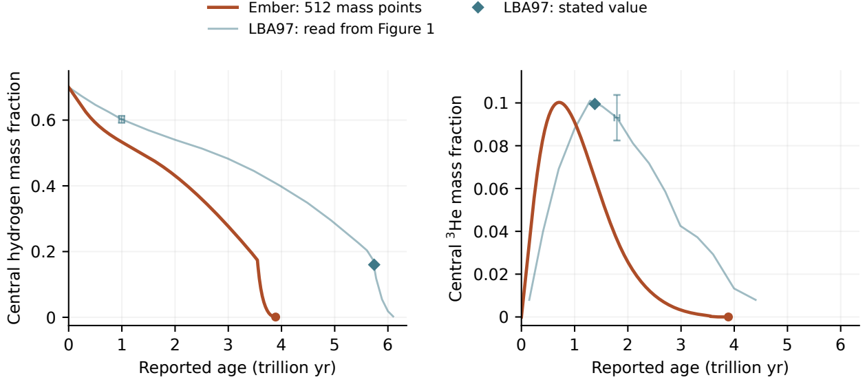
Figure 13: Hydrogen consumption and the buildup and depletion of ^3\text{He} in the pp comparison without microscopic separation. The pale curves are read from the inset of LBA97 Figure 1, with 20 hydrogen and 15 helium-3 samples. Diamonds show their stated ^3\text{He} maximum and the hydrogen abundance at central radiative-core formation. Orange curves are the 512-point Ember track through 3.890Tyr. Ages are shown as reported, without shifting or stretching either calculation. The representative crosses correspond to four image pixels: about 0.05Tyr in age and 0.01 in mass fraction. They illustrate reading precision, not statistical or physical uncertainty. The rapid final hydrogen decline is poorly resolved in the printed inset; the helium-3 trace ends as it becomes indistinguishable from the baseline.
