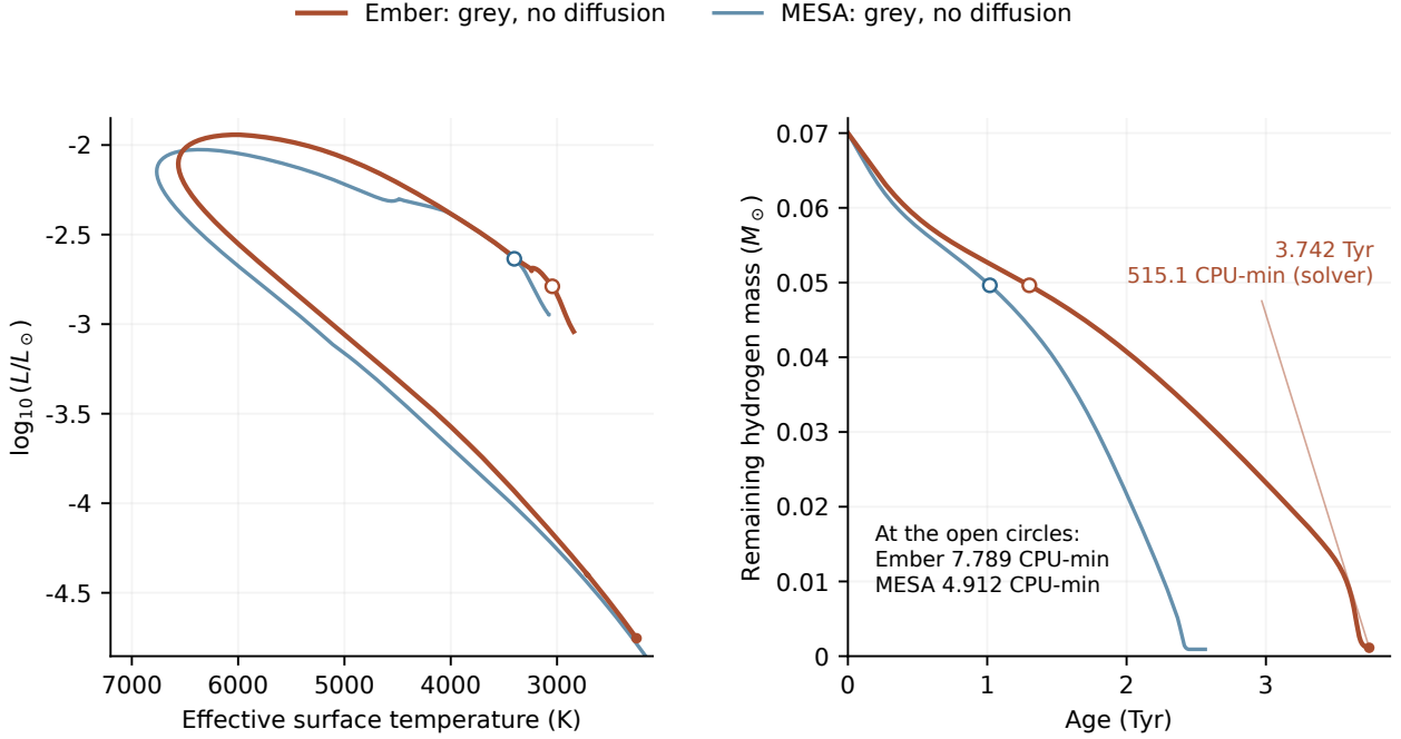
Figure 11: Grey-atmosphere calculations without microscopic diffusion. Both have initial mass 0.1M_{\odot} , X = 0.7 and Z = 0.02 . Orange is Ember through 3.742Tyr; blue is MESA. Open circles mark the same remaining hydrogen mass, 0.04963M_{\odot} , used for the CPU comparison. The filled orange point marks the last computed Ember model in this figure; its label gives the cumulative 515.1 solver CPU-minutes for that sequence. The open-circle times refer only to the earlier equal-hydrogen comparison. The equations of state, opacities and reaction networks differ. CPU times have the scope defined in the text and are summed over evaluation threads. MESA’s age includes contraction; Ember starts from a static hydrogen-burning model. The small Ember luminosity dip near 3241 K accompanies the loss of full convection. The MESA cooling branch continues beyond the displayed H–R limits.
