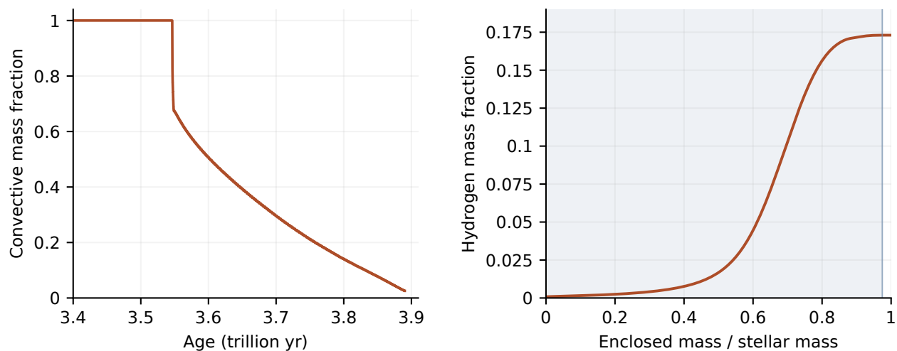
Figure 14: Convection and chemical separation by nuclear burning and macroscopic mixing in the pp comparison without microscopic separation. Left: the fraction of mass in convective regions declines from unity near 3.546Tyr to 0.02565 at 3.890Tyr. Right: the hydrogen profile in the 3.890Tyr model. The shaded core carries heat by radiation and conduction; the outer convective envelope has an almost uniform hydrogen abundance. Both panels use the same calculation and its final saved structure.
