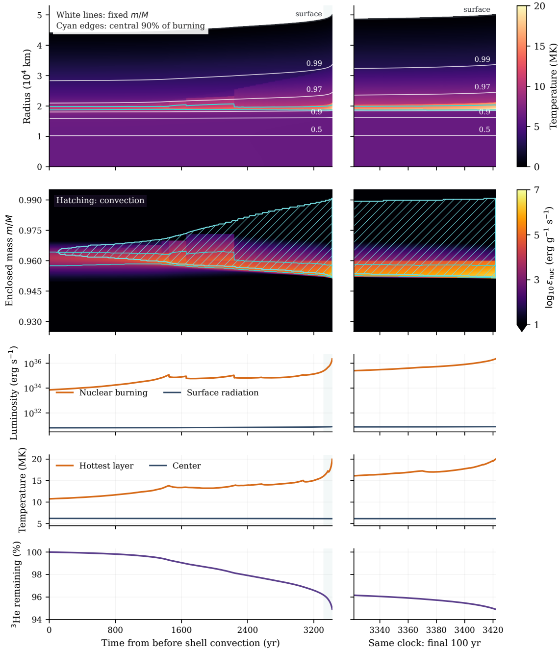
Figure 8: Internal development of the helium-3 pulse on the 666-point grid. The left column spans the computed interval; the right enlarges its final 100 yr on the same clock. Upper panel: temperature versus radius, with white curves following fixed enclosed mass fractions and cyan curves bounding the central 90% of nuclear power. Second panel: specific nuclear heating versus enclosed mass, with connected convective regions hatched. Lower panels show luminosities, temperatures and remaining helium-3. Time zero is an already-burning model before shell convection. The sequence ends during a renewed rise; the final peak and shutdown remain undetermined. The spatial sensitivity is shown in Figure 7.
