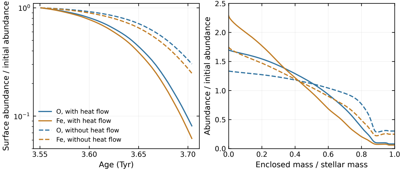
Figure 9: Passive oxygen and iron redistribution on prescribed stellar structures. Left: surface abundance relative to its initial value. Right: the abundance profile at 3.704Tyr. Solid curves include classical heat flow; dashed curves suppress it. Each tracer’s total inventory is conserved, and the changing convective envelope is mixed by mass. The two heat-flow treatments do not define an uncertainty band, and neither includes the star’s response to the changing metal opacity.
