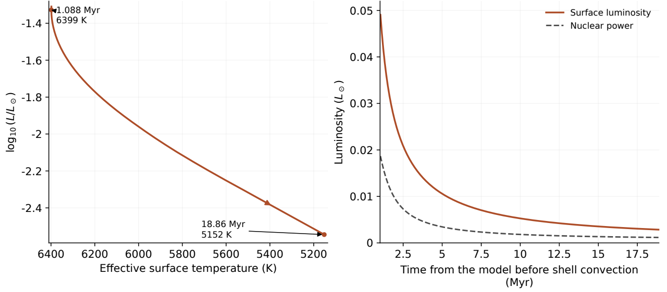
Figure 6: The late shell-burning calculation on 2115 mass points. Left: an enlarged HR diagram around the effective-temperature maximum. The arrow follows increasing time. Right: photon luminosity and deposited nuclear power over the same interval. Time is measured from the model before shell convection. Temperature declines from 6399 K to 5152 K over 1.777 \times 10^7 yr; nuclear burning supplies 40.96% of the final surface luminosity. The contracting model has turned toward cooling. Its physical connection to the calculation resolving the flash from its onset remains unverified.
